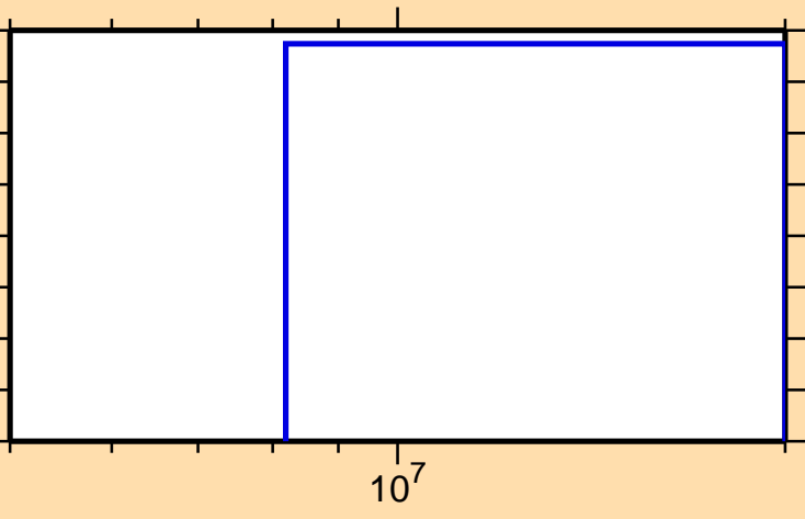
\sigma vs. E for ^{231}\text{U}(n,\text{nd})
