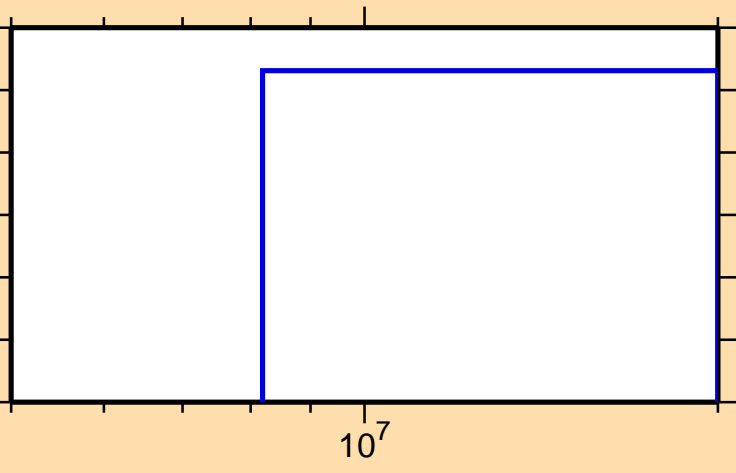
\sigma vs. E for ^{231}\text{U}(n,3n)
