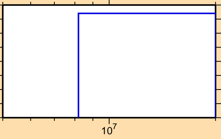
\sigma vs. E for ^{231}\text{U} (mt 42)
