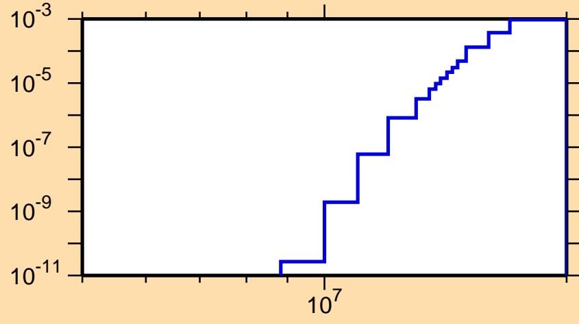
\sigma vs. E for ^{234}\text{U}(n,d)
