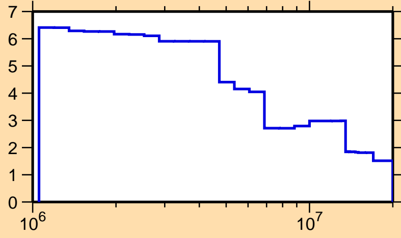
\Delta\sigma/\sigma vs. E for ^{234}\text{U}(n, nonel.)
