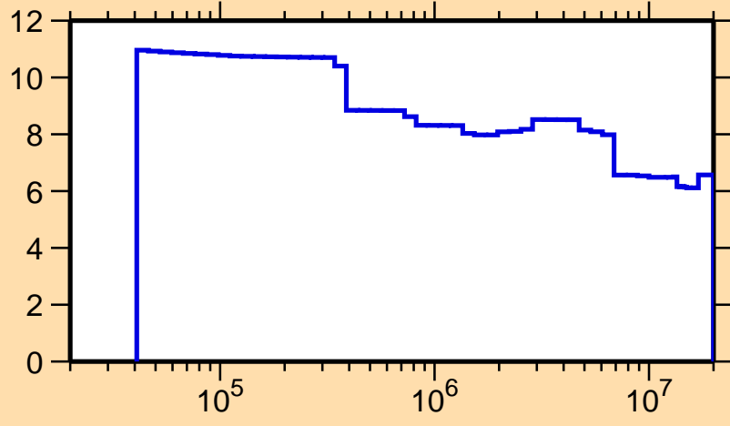
\Delta\sigma/\sigma vs. E for ^{234}\text{U}(n,\text{tot.})
