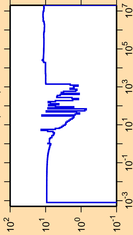
\Delta\sigma/\sigma vs. E for ^{234}\text{U}(n,\text{el.})
