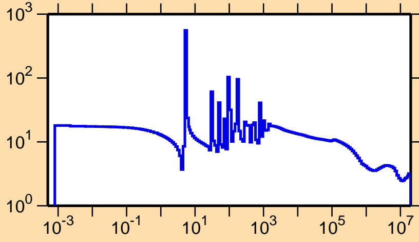
\sigma vs. E for ^{234}\text{U}(n,\text{el.})
