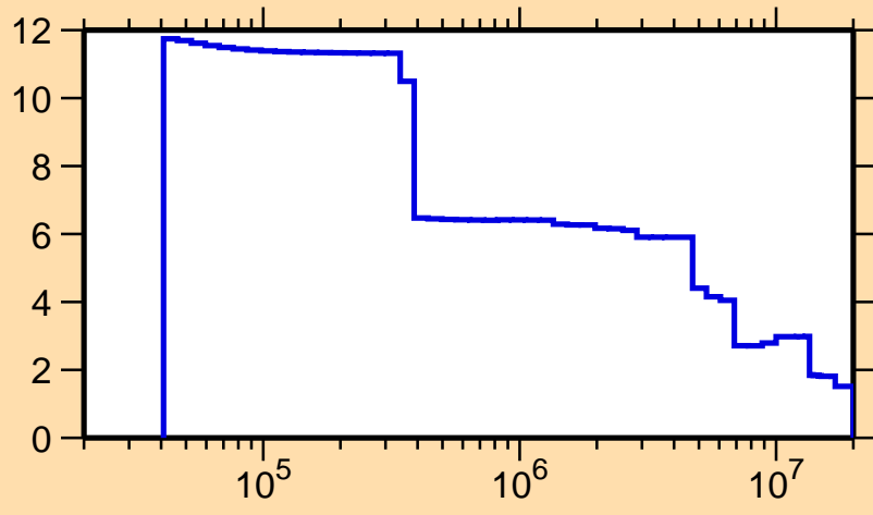
\Delta\sigma/\sigma vs. E for ^{234}\text{U}(n,\text{nonel.})
