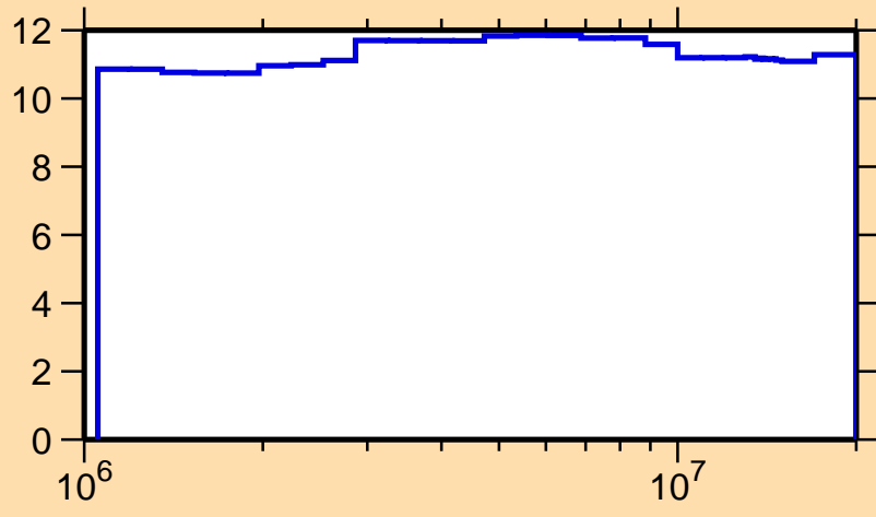
\Delta\sigma/\sigma vs. E for ^{234}\text{U}(n, el.)
