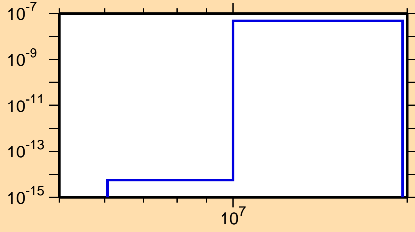
\sigma vs. E for ^{234}\text{U}(n,2n\alpha)
