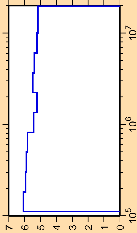
\Delta\sigma/\sigma vs. E for ^{234}\text{U}(n,n_2)
