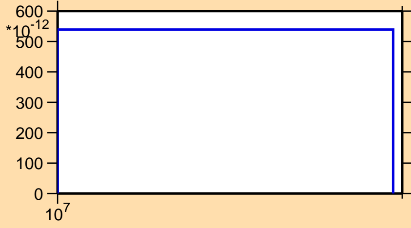
\sigma vs. E for ^{234}\text{U}(n,nd)
