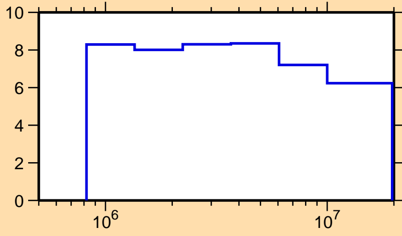
\Delta\sigma/\sigma vs. E for ^{234}\text{U}(n,tot.)
