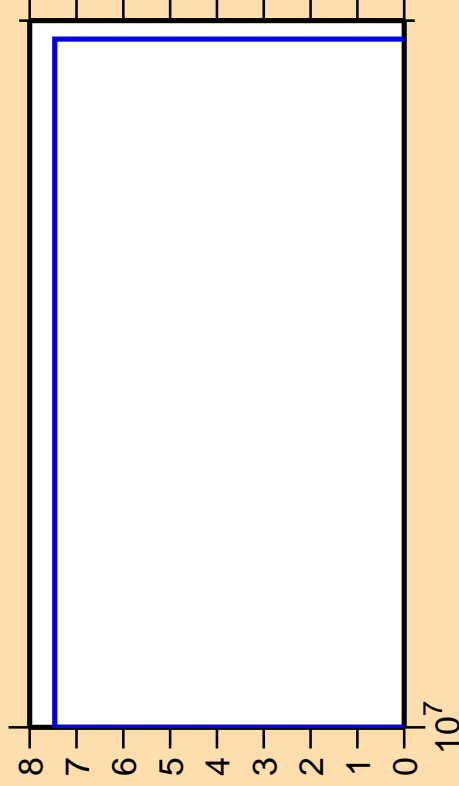
\Delta\sigma/\sigma vs. E for ^{234}\text{U}(n,2np)
