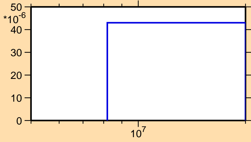
\sigma vs. E for ^{234}\text{U}(n,np)
