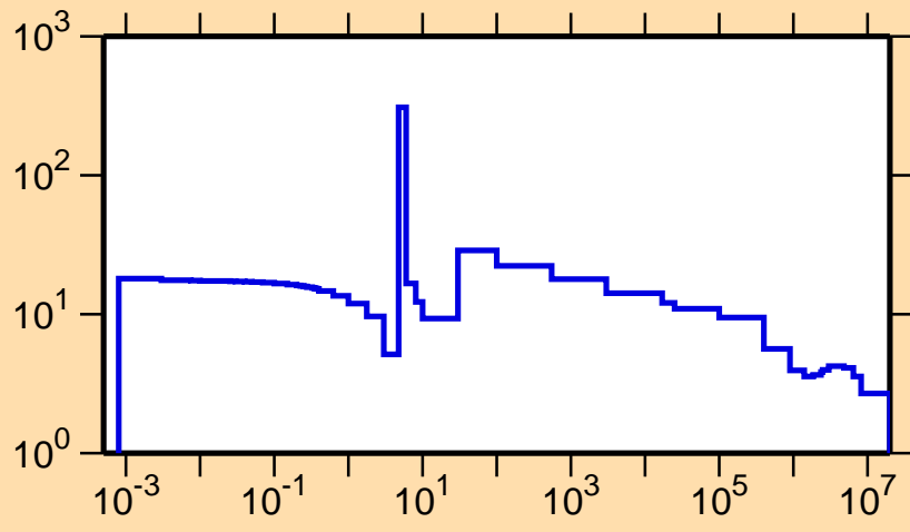
\sigma vs. E for ^{234}\text{U}(n,\text{el.})
