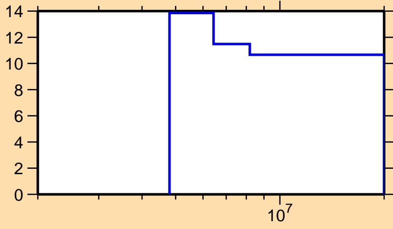
\Delta\sigma/\sigma vs. E for ^{234}\text{U}(n,inel.)
