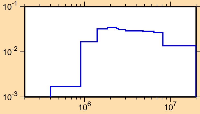
\sigma vs. E for ^{234}\text{U}(n,n_3)
