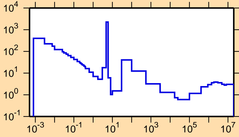
\sigma vs. E for ^{234}\text{U}(n,\text{nonel.})
