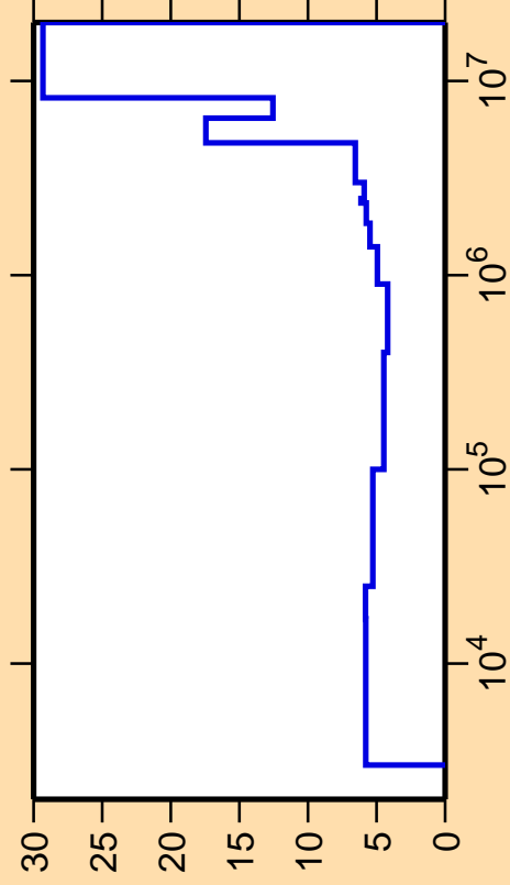
\Delta\sigma/\sigma vs. E for ^{235}\text{U} (mt852)
