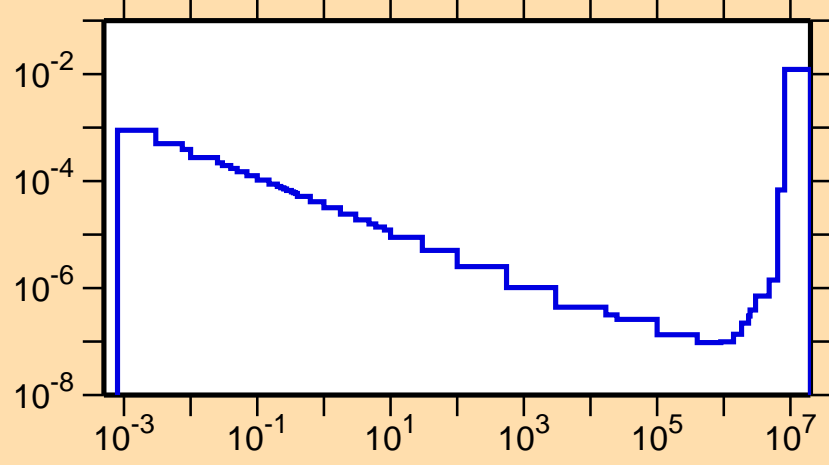
\sigma vs. E for ^{235}\text{U} (mt 5)
