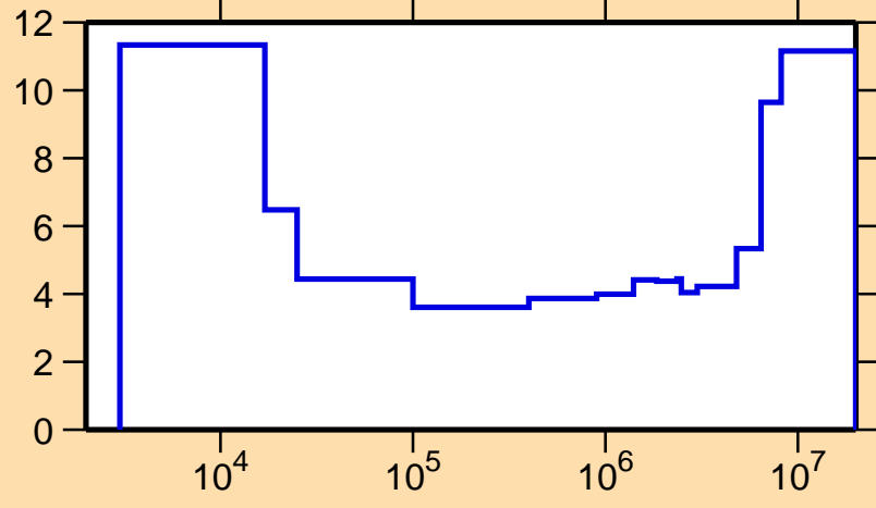
\Delta\sigma/\sigma vs. E for ^{235}\text{U} (mt851)
