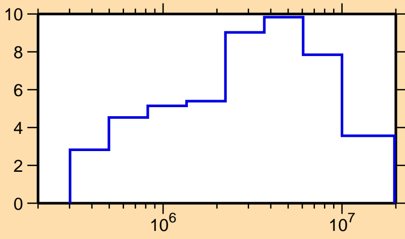
\Delta\sigma/\sigma vs. E for ^{235}\text{U}(n, tot.)
