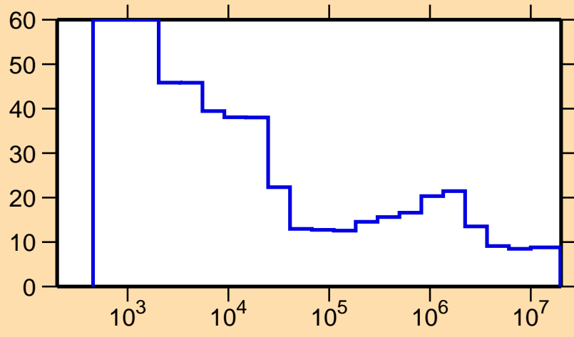
\Delta\sigma/\sigma vs. E for ^{235}\text{U}(n,\text{nonel.})
