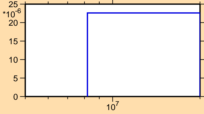
\sigma vs. E for ^{235}\text{U}(n,np)
