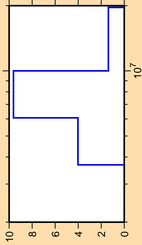
\Delta\sigma/\sigma vs. E for ^{236}\text{U}(n,n\alpha)
