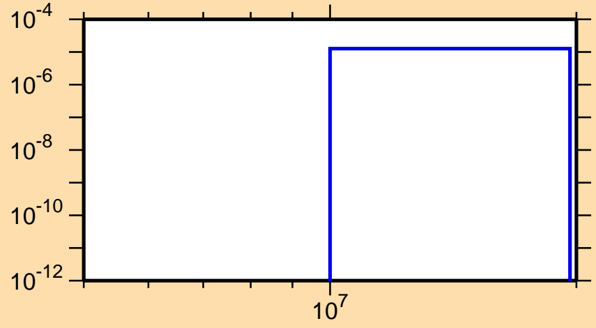
\sigma vs. E for ^{236}\text{U}(n,t)
