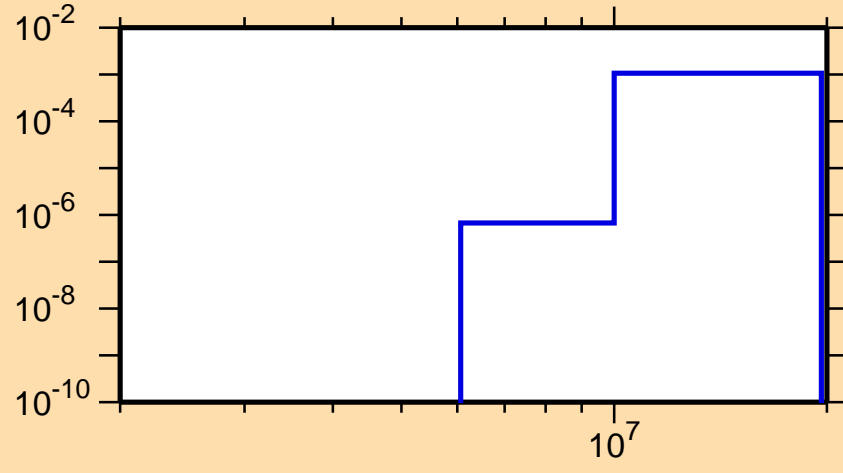
\sigma vs. E for ^{237}\text{U}(n,p)
