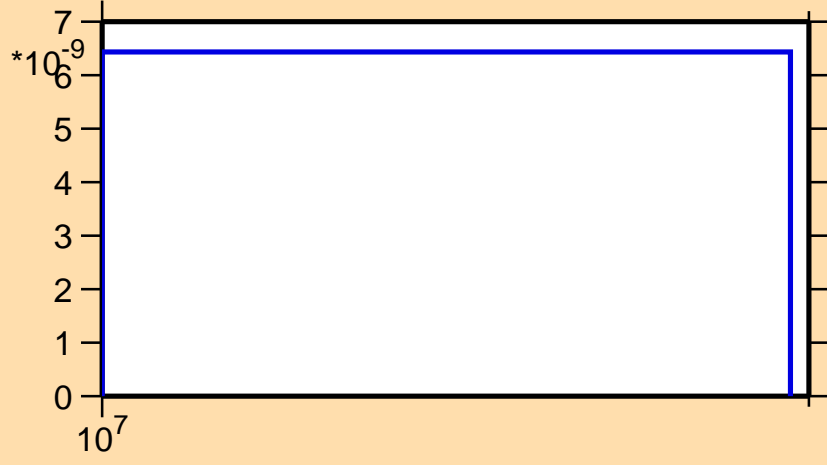
\sigma vs. E for ^{237}\text{U}(n,2n\alpha)
