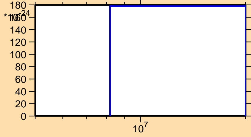
\sigma vs. E for ^{237}\text{U} (mt 42)
