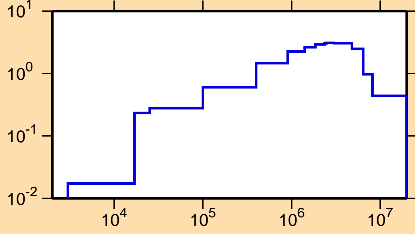
\sigma vs. E for ^{237}\text{U}(n,\text{inel.})
