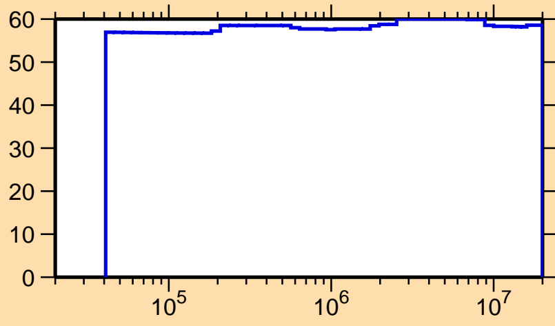
\Delta\sigma/\sigma vs. E for ^{239}\text{U}(n,\text{el.})
