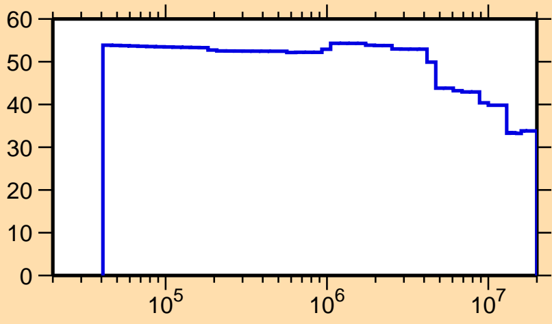
\Delta\sigma/\sigma vs. E for ^{239}\text{U}(n,\text{tot.})
