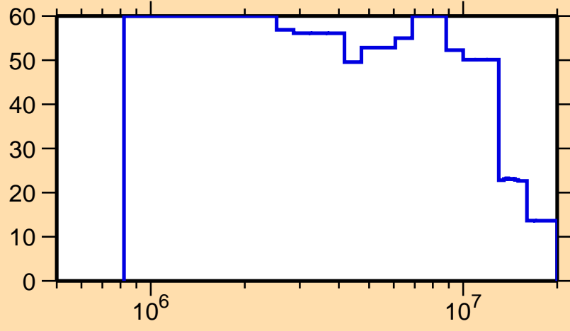
\Delta\sigma/\sigma vs. E for ^{239}\text{U}(n, nonel.)
