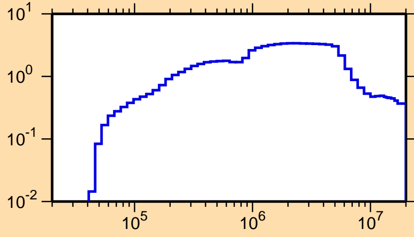
\sigma vs. E for ^{239}\text{U}(n,\text{inel.})
