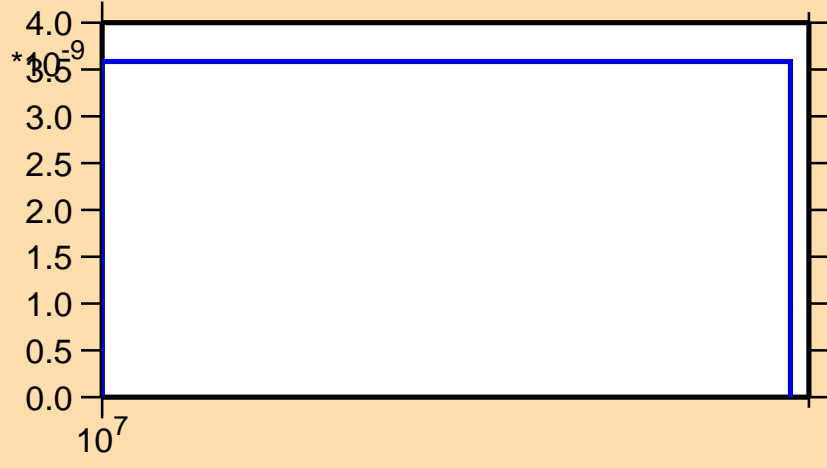
\sigma vs. E for ^{239}\text{U}(n,nd)
