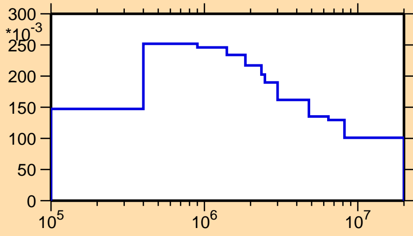
\sigma vs. E for ^{239}\text{U}(n,n_2)
