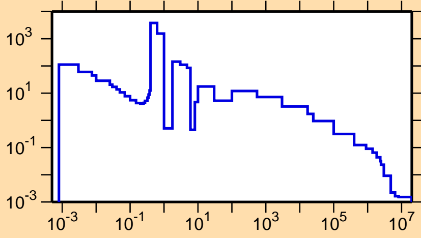
\sigma vs. E for ^{239}\text{U}(n,\gamma)
