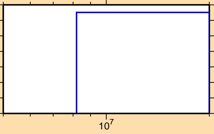
\sigma vs. E for ^{239}\text{U}(n,nd)
