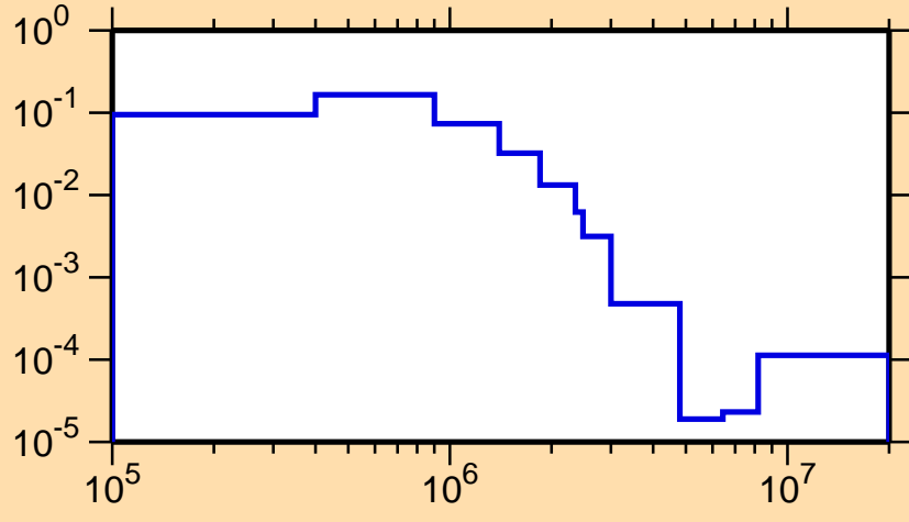
\sigma vs. E for ^{239}\text{U}(n,n_4)
