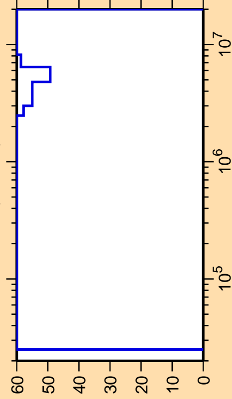
\Delta\sigma/\sigma vs. E for ^{239}\text{U}(n,\text{inel.})
