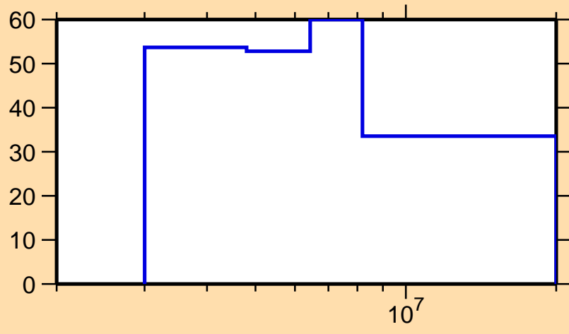
\Delta\sigma/\sigma vs. E for ^{239}\text{U}(n,\text{nonel.})
