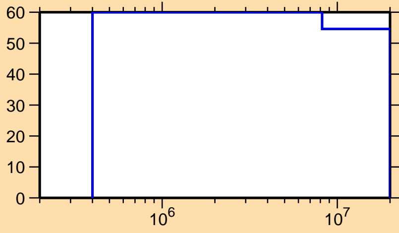
\Delta\sigma/\sigma vs. E for ^{239}\text{U}(n,\text{f})
