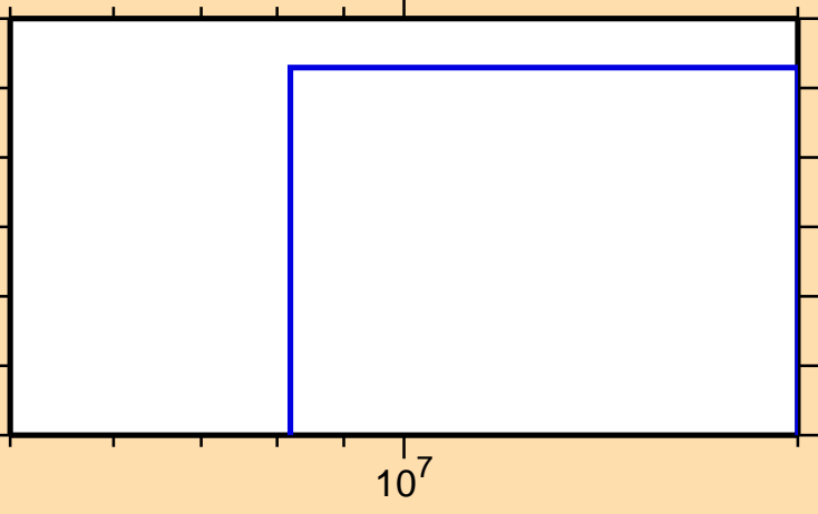
\sigma vs. E for ^{239}\text{U}(n,2n\alpha)
