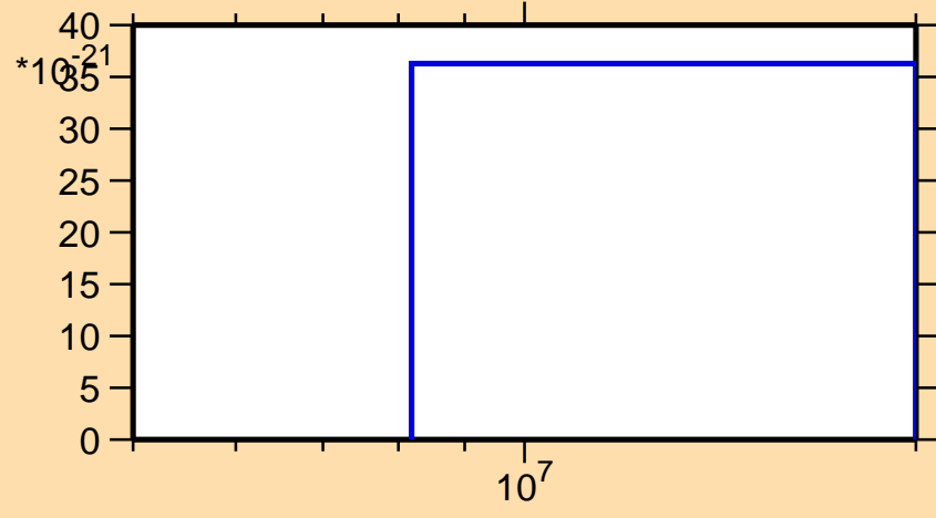
\sigma vs. E for ^{239}\text{U} (mt 42)
