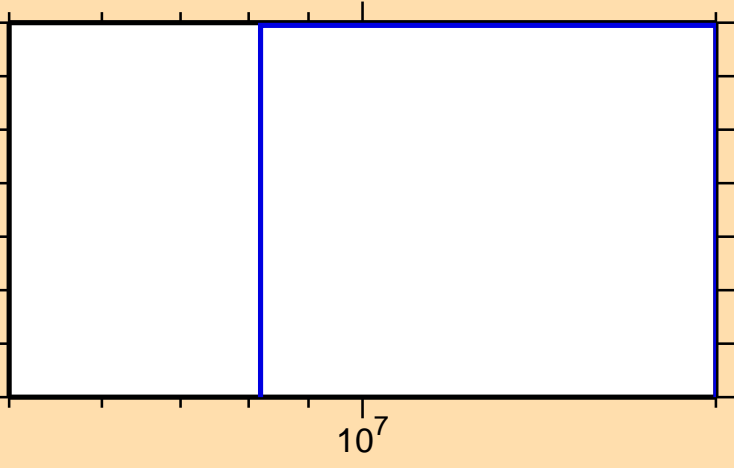
\sigma vs. E for ^{239}\text{U}(n,np)
