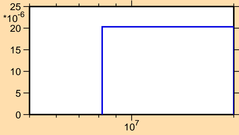
\sigma vs. E for ^{239}\text{U}(n,d)
