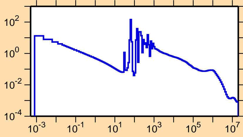
\sigma vs. E for ^{240}\text{U}(n,\gamma)
