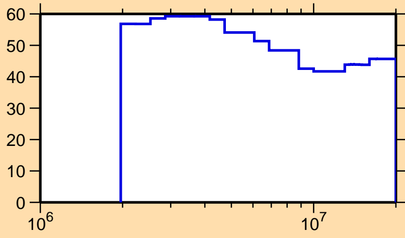
\Delta\sigma/\sigma vs. E for ^{240}\text{U}(n, tot.)
