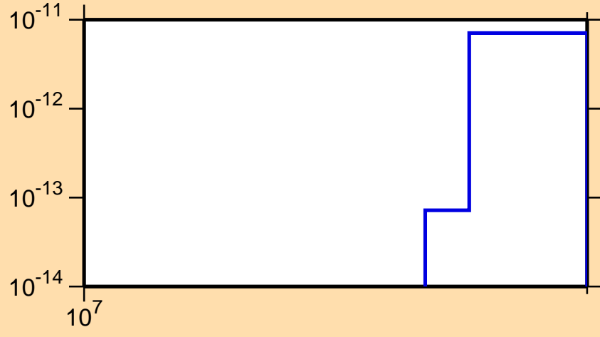
\sigma vs. E for ^{240}\text{U}(n,3n\alpha)
