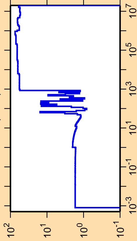
\Delta\sigma/\sigma vs. E for ^{240}\text{U}(n,\text{el.})
