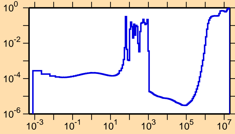
\sigma vs. E for ^{240}\text{U}(n,f)
