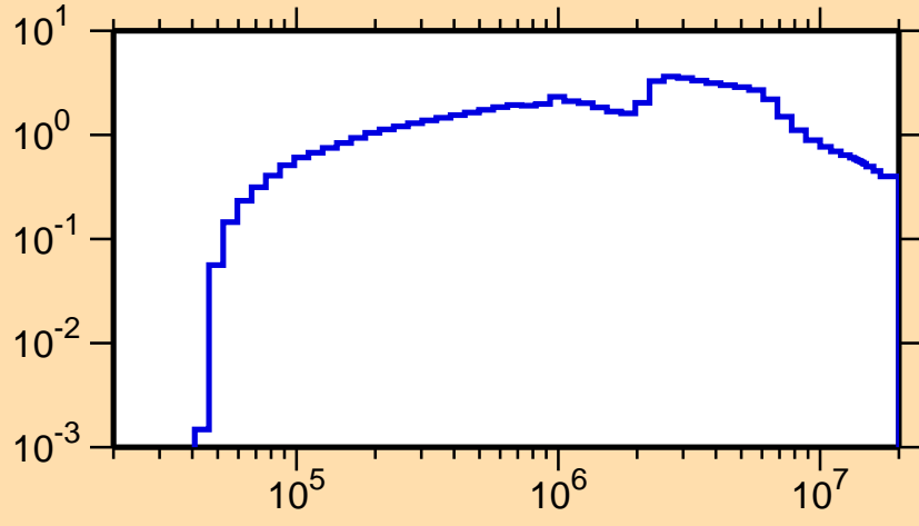
\sigma vs. E for ^{240}\text{U}(n,\text{inel.})
