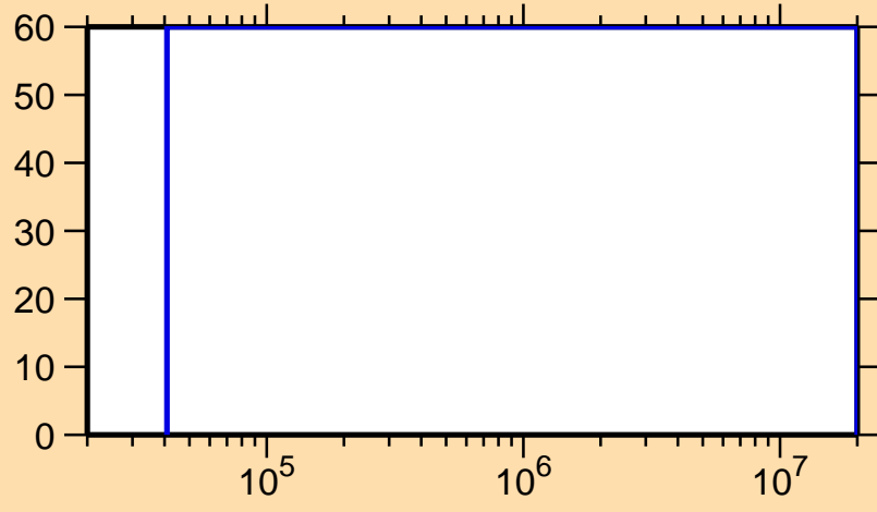
\Delta\sigma/\sigma vs. E for ^{240}\text{U}(n,f)
