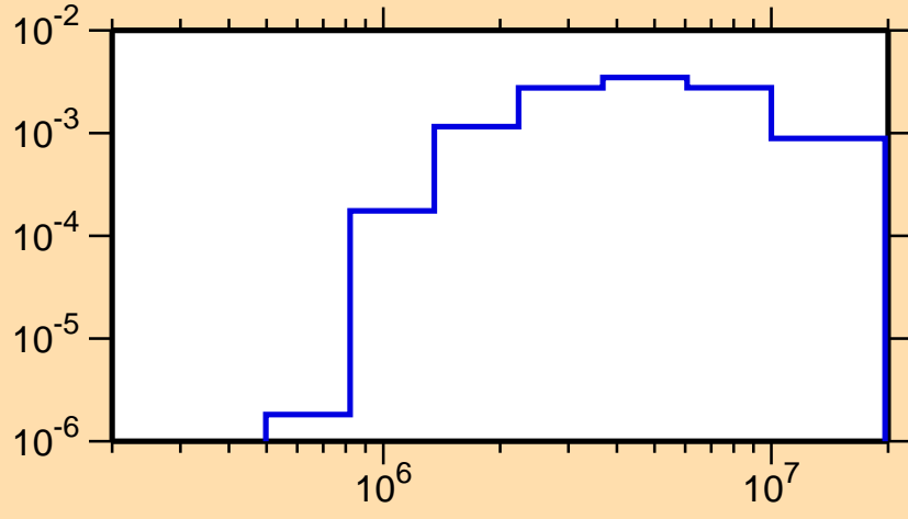
\sigma vs. E for ^{240}\text{U}(n,n_4)
