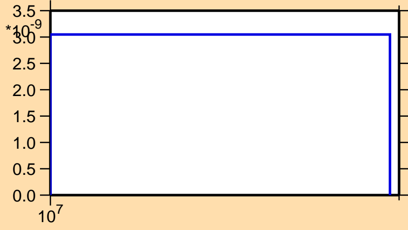
\sigma vs. E for ^{240}\text{U}(n,nt)
