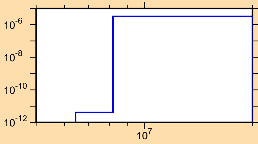
\sigma vs. E for ^{240}\text{U}(n,n\alpha)
