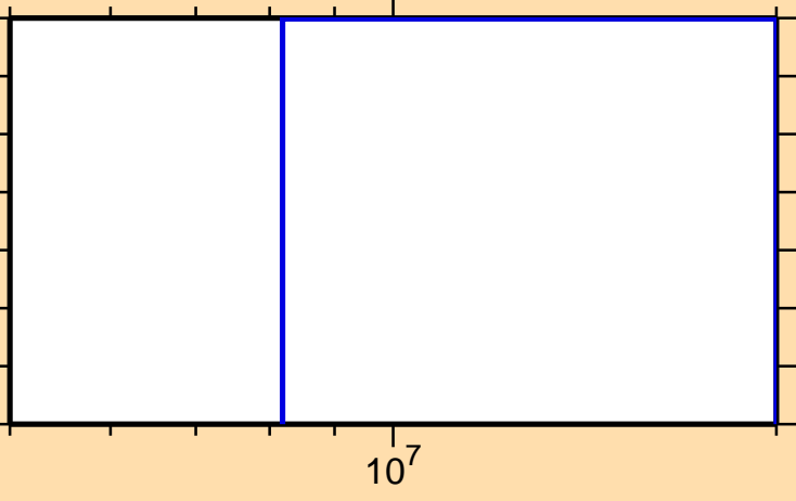
\sigma vs. E for ^{240}\text{U}(n,d)
