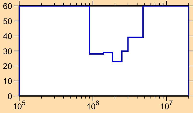
\Delta\sigma/\sigma vs. E for ^{241}\text{U}(n,\text{inel.})
