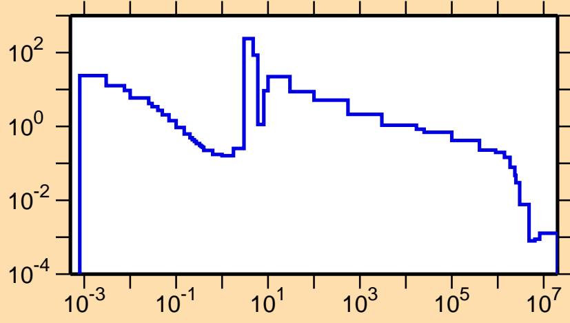
\sigma vs. E for ^{241}\text{U}(n,\gamma)
