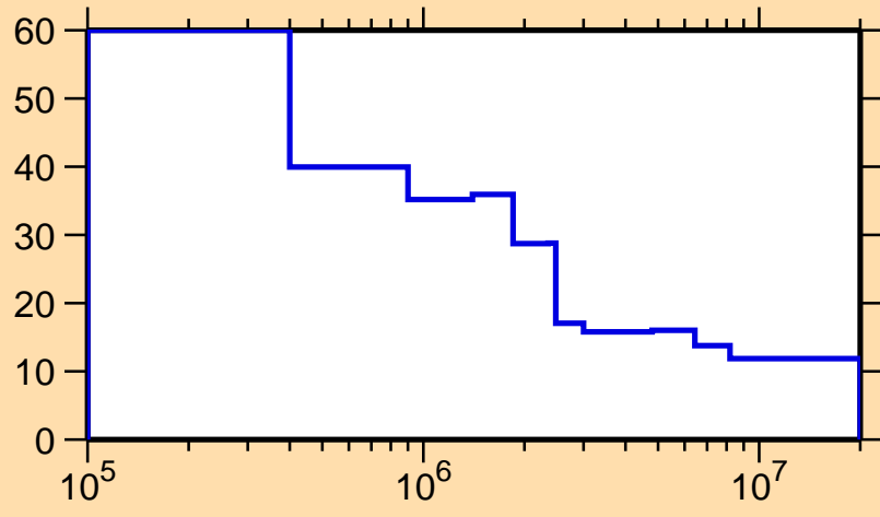
\Delta\sigma/\sigma vs. E for ^{241}\text{U}(n, nonel.)
