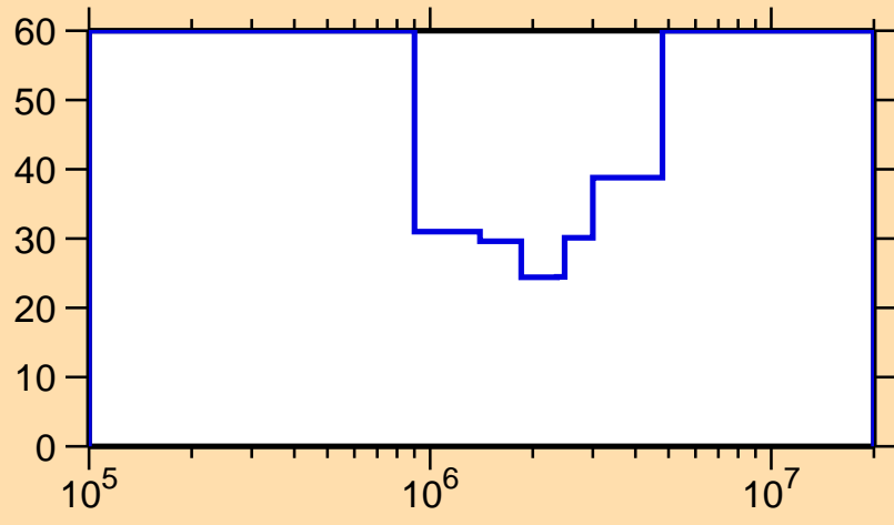
\Delta\sigma/\sigma vs. E for ^{241}\text{U}(n,n\text{cont.})
