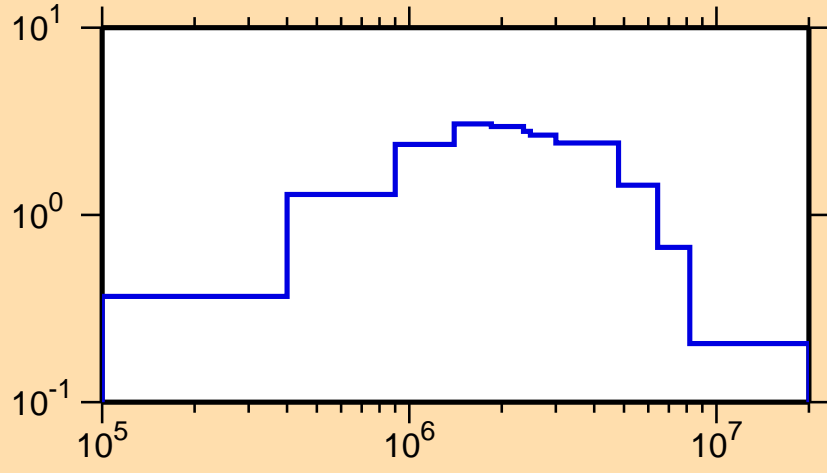
\sigma vs. E for ^{241}\text{U}(n,\text{inel.})
