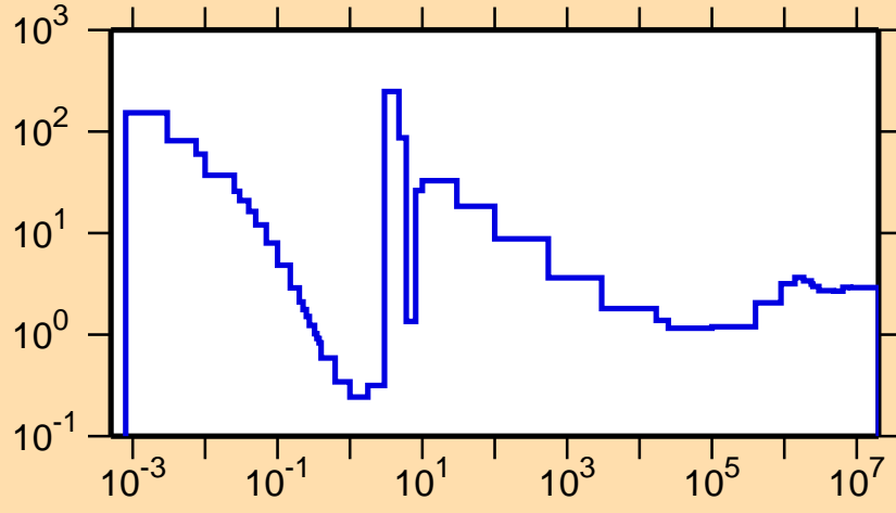
\sigma vs. E for ^{241}\text{U}(n,\text{nonel.})
