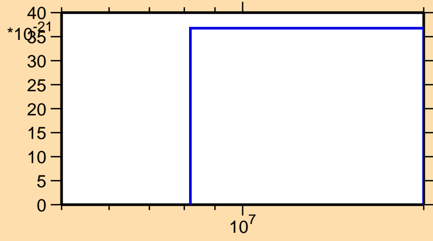
\sigma vs. E for ^{241}\text{U} (mt 42)
