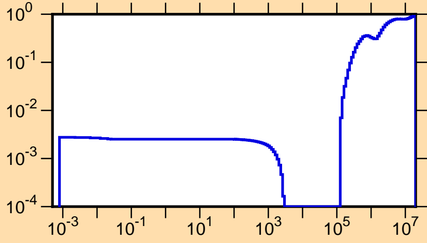
\mu vs. E for ^{242}\text{U}(\text{mt251})
