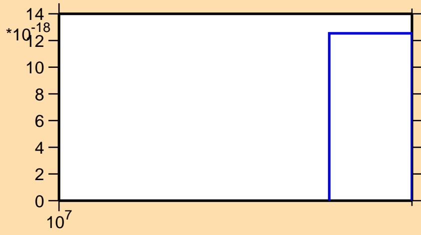
\sigma vs. E for ^{242}\text{U} (mt 42)
