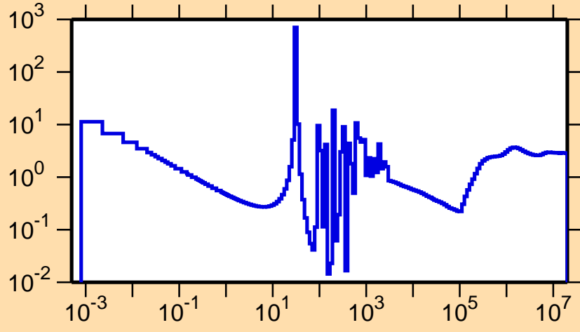
\sigma vs. E for ^{242}\text{U}(n,\text{nonel.})
