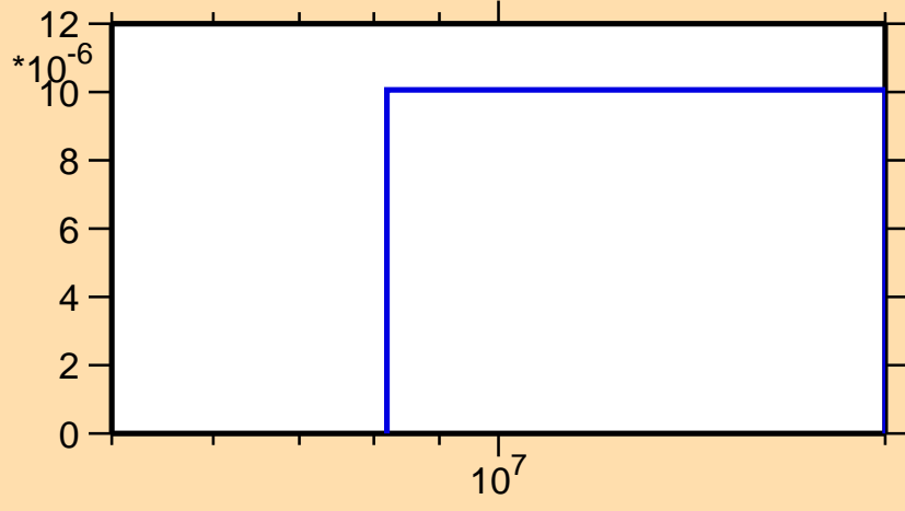
\sigma vs. E for ^{243}\text{U}(n,d)
