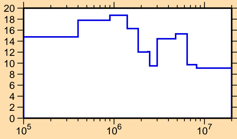
\Delta\sigma/\sigma vs. E for ^{243}\text{U}(n, tot.)
