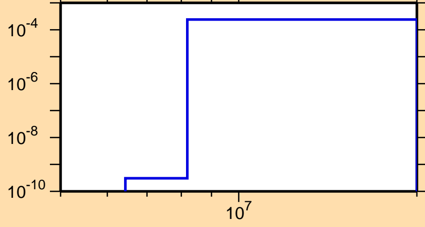
\sigma vs. E for ^{243}\text{U}(n,p)
