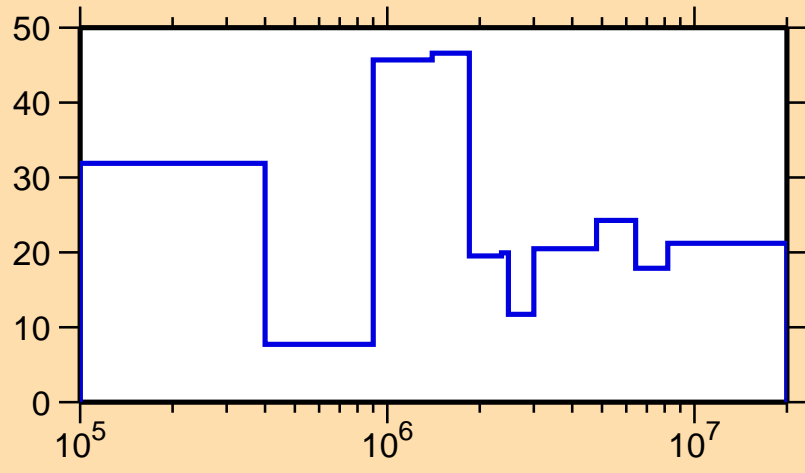
\Delta\sigma/\sigma vs. E for ^{243}\text{U}(n, el.)
