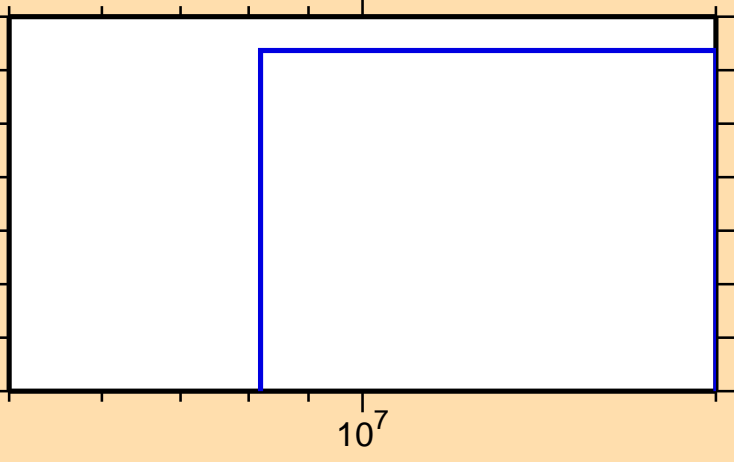
\sigma vs. E for ^{243}\text{U}(n,2n\alpha)
