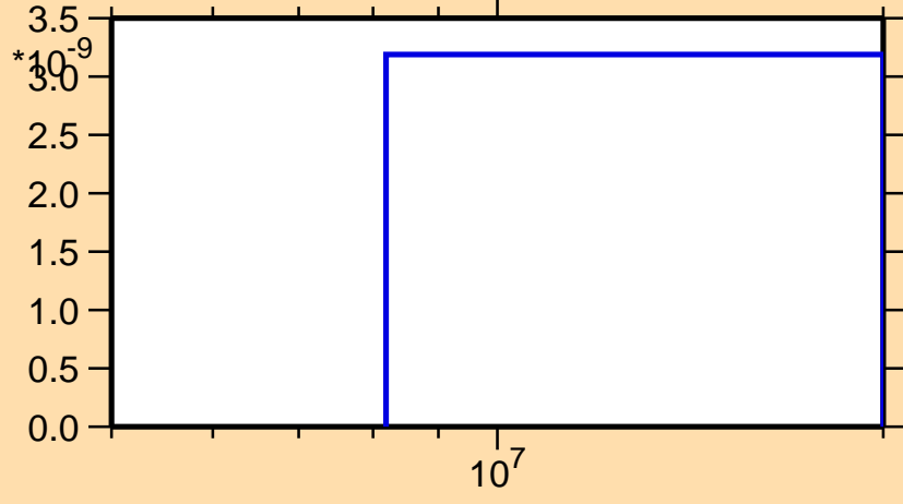
\sigma vs. E for ^{243}\text{U}(n,\text{nd})
