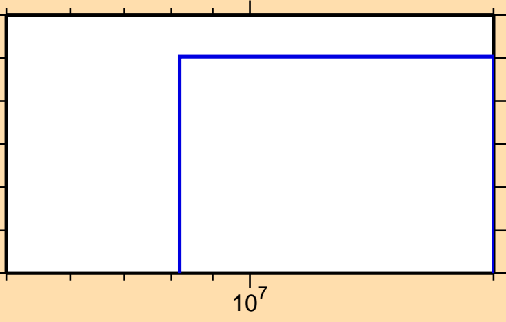
\sigma vs. E for ^{243}\text{U}(n,d)
