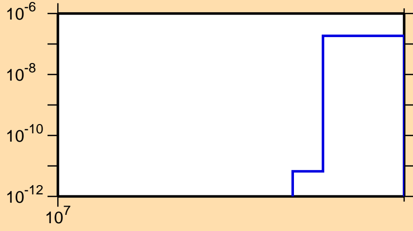
\sigma vs. E for ^{47}\text{V} (mt 45)
