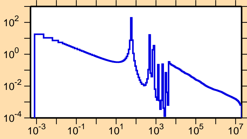
\sigma vs. E for ^{47}\text{V}(n,\gamma)
