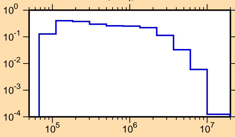
\sigma vs. E for ^{47}\text{V}(n,n_1)
