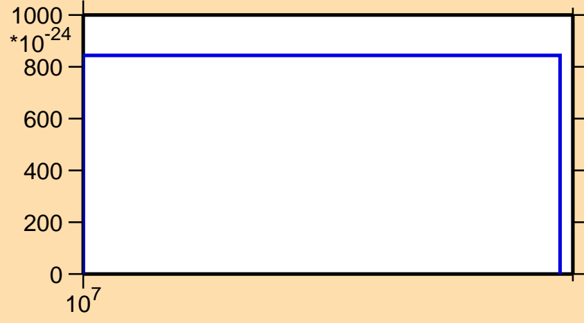
\sigma vs. E for ^{47}\text{V}(n,\text{pt})
