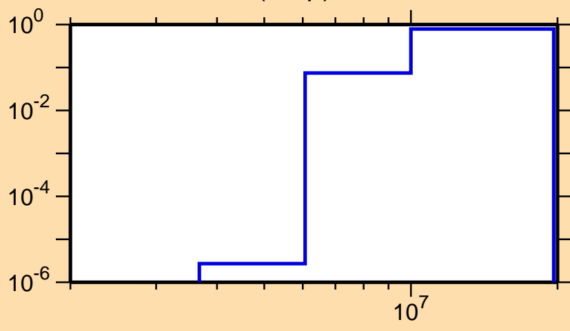
\sigma vs. E for ^{47}\text{V}(n,np)
