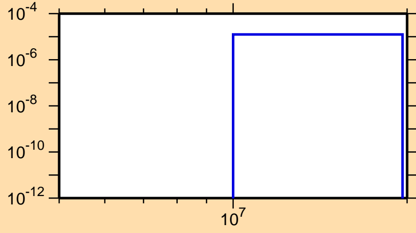
\sigma vs. E for ^{47}\text{V}(n,\text{He3})
