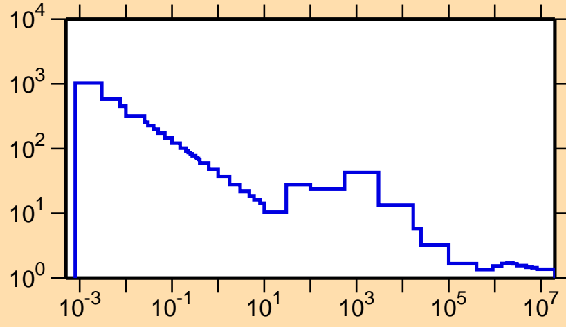
\sigma vs. E for ^{47}\text{V}(n,\text{nonel.})
