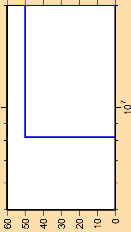
\Delta\sigma/\sigma vs. E for ^{47}\text{V}(n,n_1)
