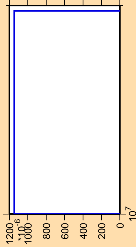
\Delta\sigma/\sigma vs. E for ^{48}\text{V}(n,\text{pt})
