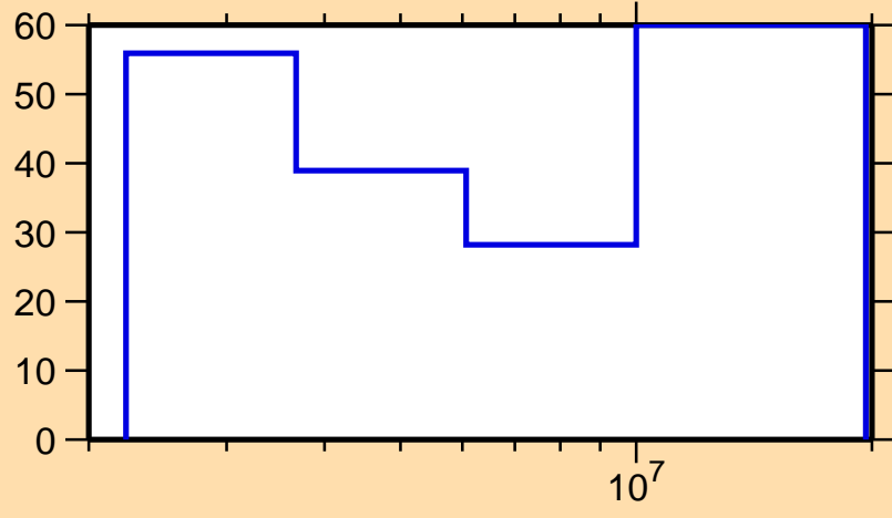
\Delta\sigma/\sigma vs. E for ^{48}\text{V}(n,n\text{cont.})
