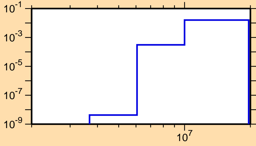
\sigma vs. E for ^{48}\text{V}(n,d)
