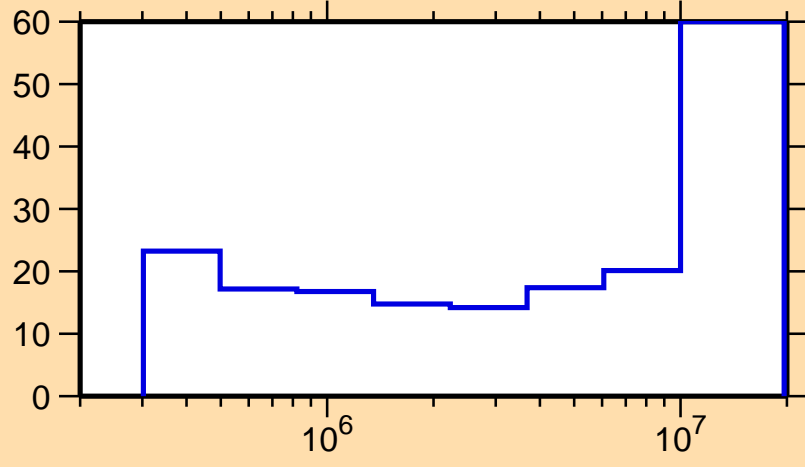
\Delta\sigma/\sigma vs. E for ^{48}\text{V}(n,\text{inel.})
