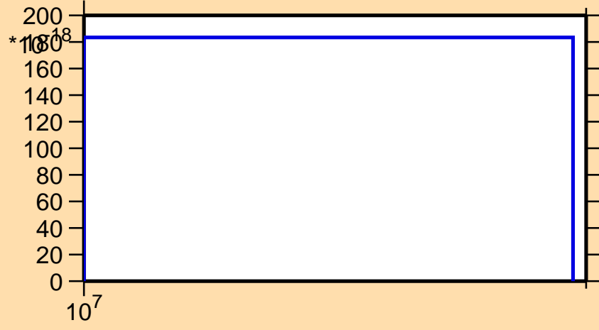
\sigma vs. E for ^{48}\text{V}(n,\text{pt})
