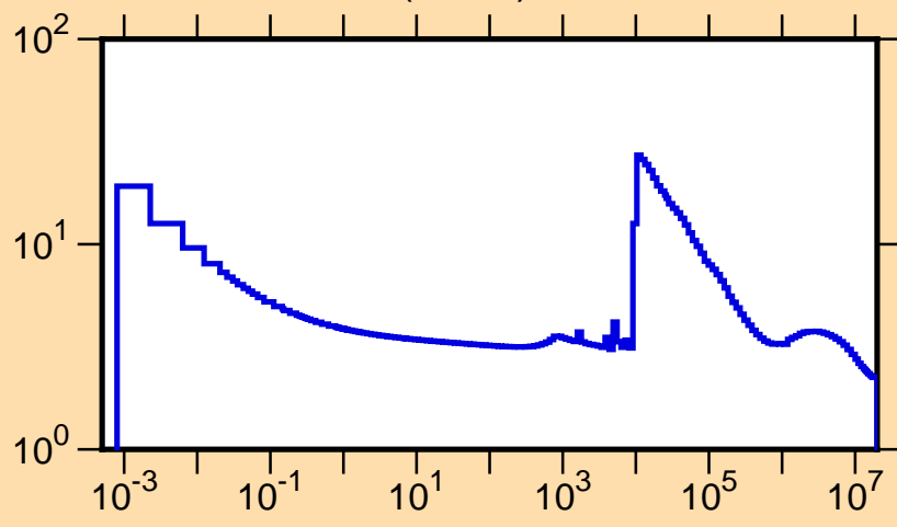
\sigma vs. E for ^{49}\text{V}(n,\text{tot.})
