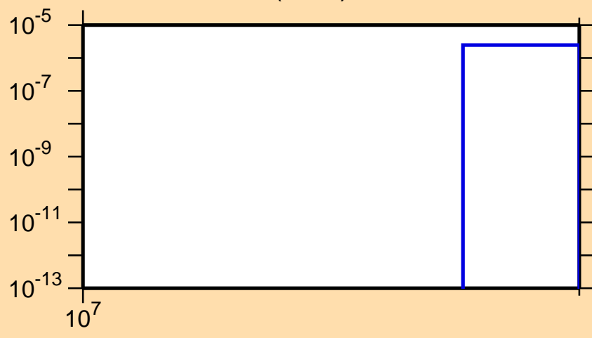
\sigma vs. E for ^{49}\text{V}(n,\text{nd})
