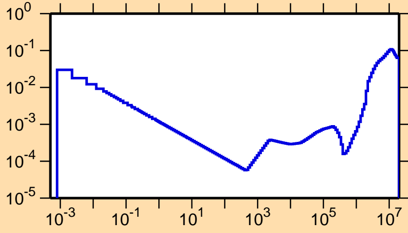
\sigma vs. E for ^{50}\text{V}(n,p)
