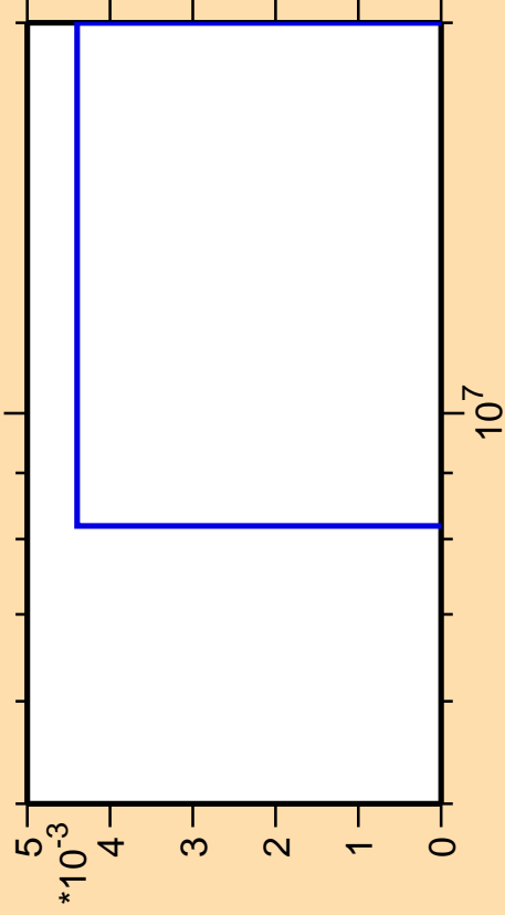
\Delta\sigma/\sigma vs. E for ^{50}\text{V}(n,\text{pd})
