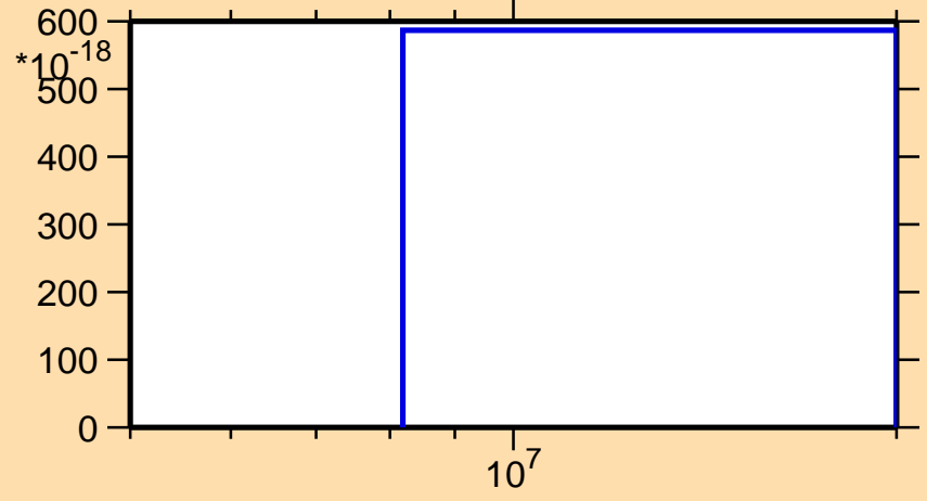
\sigma vs. E for ^{50}\text{V}(n,\text{pd})
