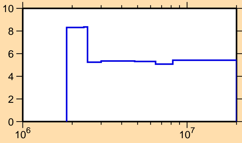
\Delta\sigma/\sigma vs. E for ^{50}\text{V}(n, n\text{onel.})
