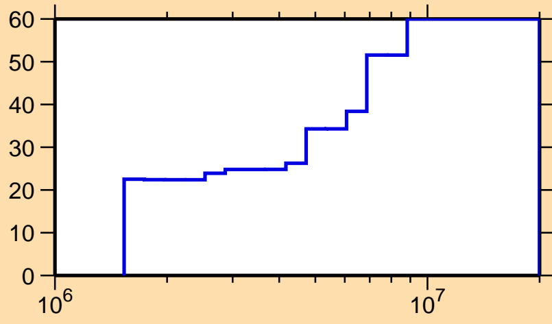
\Delta\sigma/\sigma vs. E for ^{51}\text{V}(n,\gamma)
