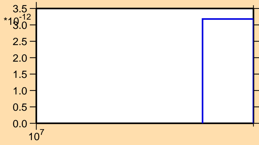
\sigma vs. E for ^{51}\text{V}(n,2np)
