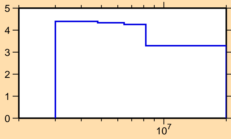
\Delta\sigma/\sigma vs. E for ^{51}\text{V}(n,tot.)
