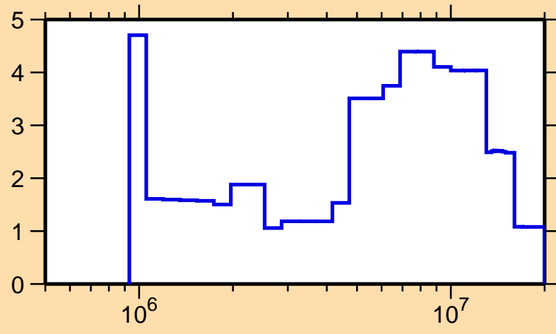
\Delta\sigma/\sigma vs. E for ^{52}\text{V}(n,\text{tot.})
