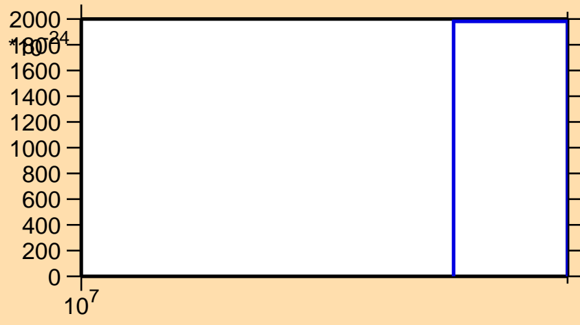
\sigma vs. E for ^{52}\text{V}(n,\text{pt})
