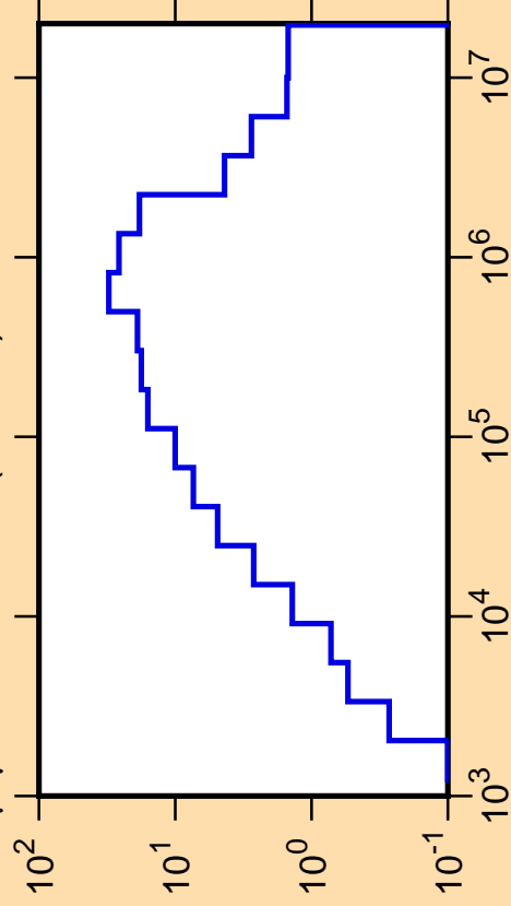
\Delta\mu/\mu vs. E for ^{52}\text{V}(\text{mt251})
