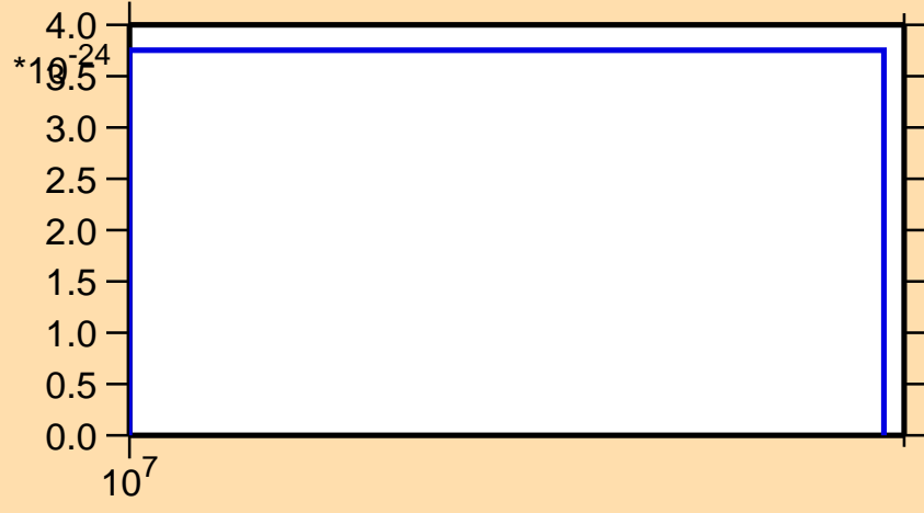
\sigma vs. E for ^{52}\text{V}(n,\text{pt})
