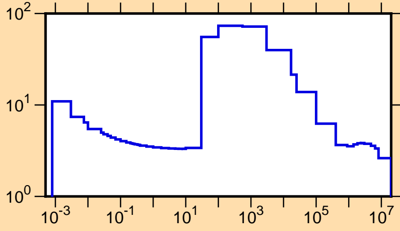
\sigma vs. E for ^{52}\text{V}(n,\text{tot.})
