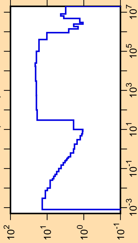
\Delta\sigma/\sigma vs. E for ^{52}\text{V}(n,\text{tot.})
