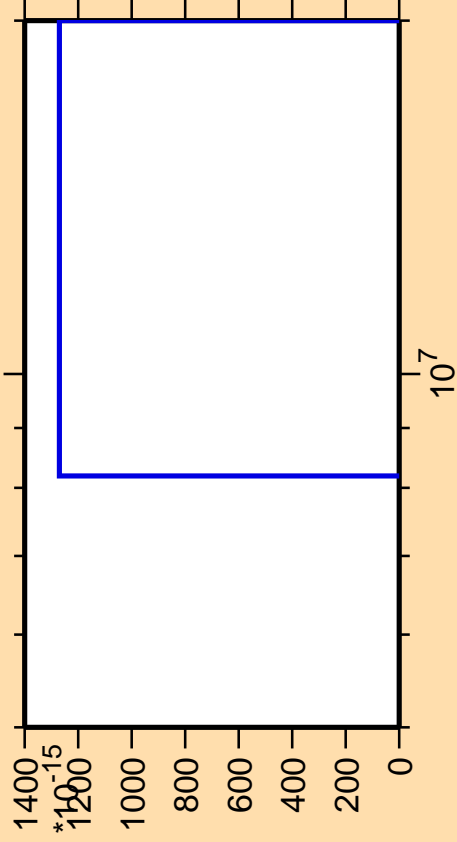
\Delta\sigma/\sigma vs. E for ^{52}\text{V}(n,pd)
