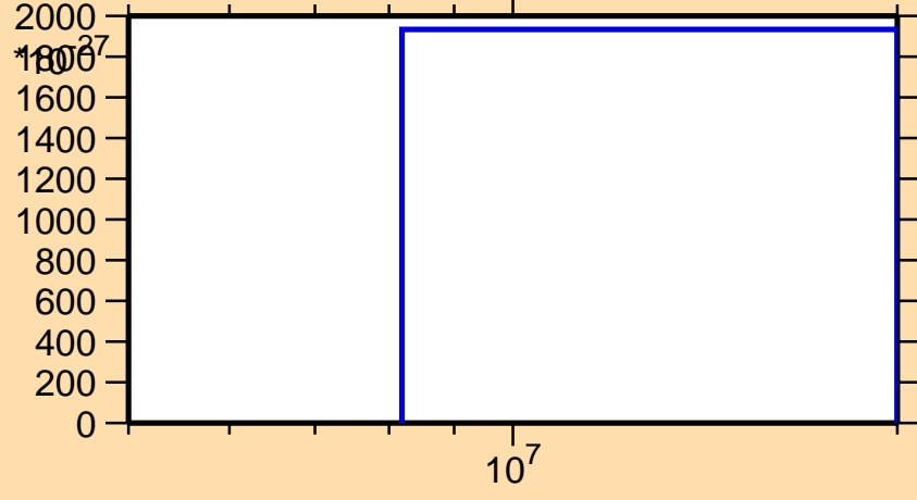
\sigma vs. E for ^{52}\text{V}(n,pd)
