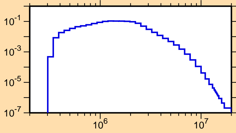
\sigma vs. E for ^{55}\text{V}(n,n_1)
