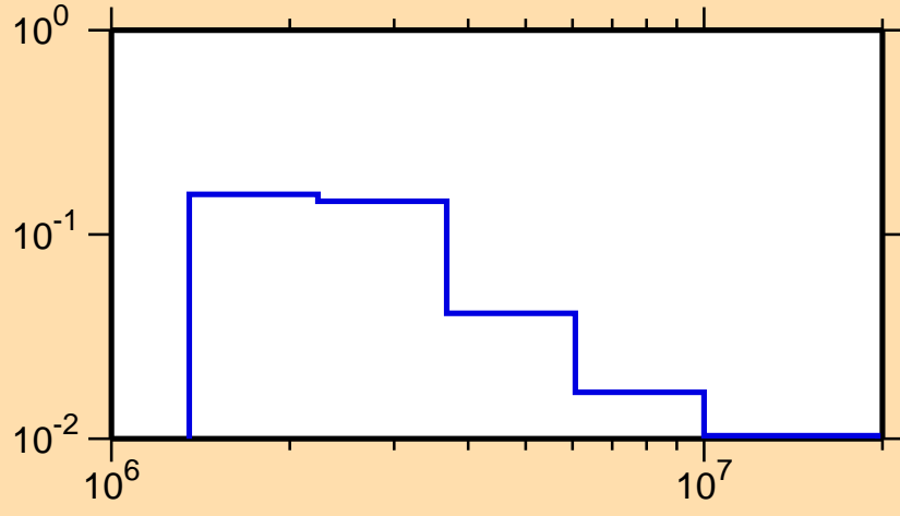
\sigma vs. E for ^{55}\text{V}(n,n_3)
