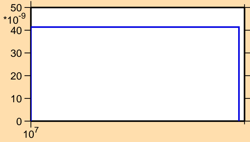
\sigma vs. E for ^{55}\text{V}(n,nd)
