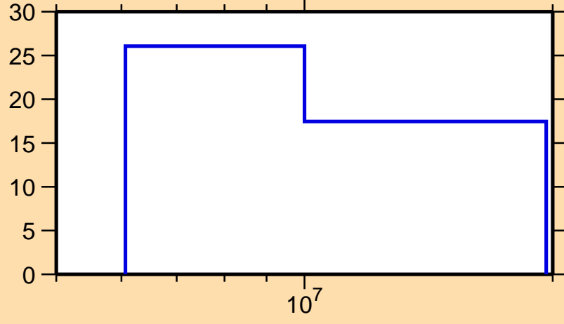
\Delta\sigma/\sigma vs. E for ^{55}\text{V}(n,2n)
