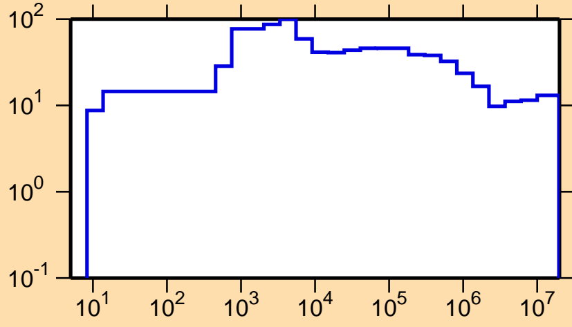
\Delta\sigma/\sigma vs. E for ^{55}\text{V}(n,\text{nonel.})
