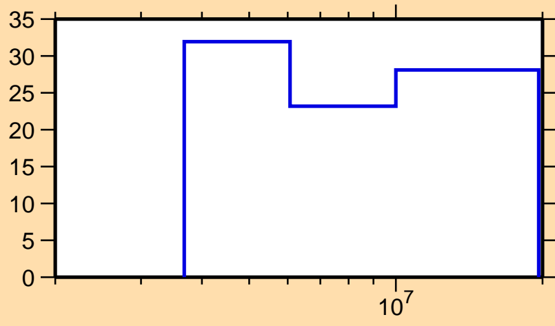
\Delta\sigma/\sigma vs. E for ^{55}\text{V}(n,n\text{cont.})
