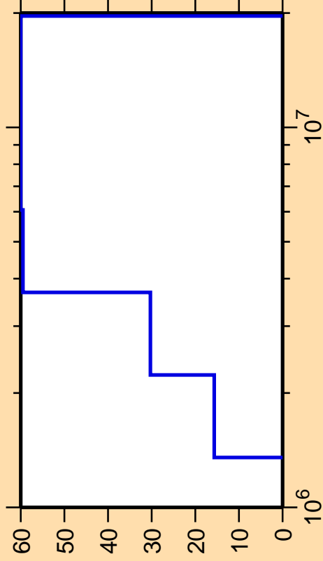
\Delta\sigma/\sigma vs. E for ^{55}\text{V}(n,n_3)
