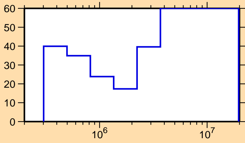
\Delta\sigma/\sigma vs. E for ^{55}\text{V}(n,n_1)
