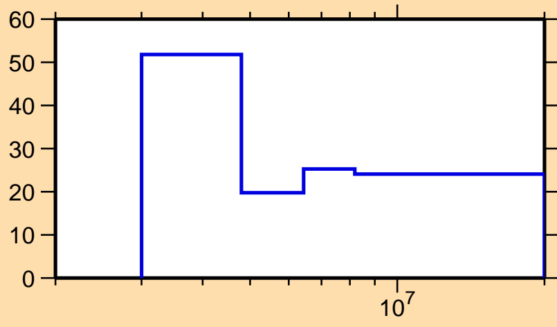
\Delta\sigma/\sigma vs. E for ^{55}\text{V}(n,ncont.)
