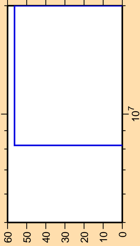
\Delta\sigma/\sigma vs. E for ^{55}\text{V}(n,d)
