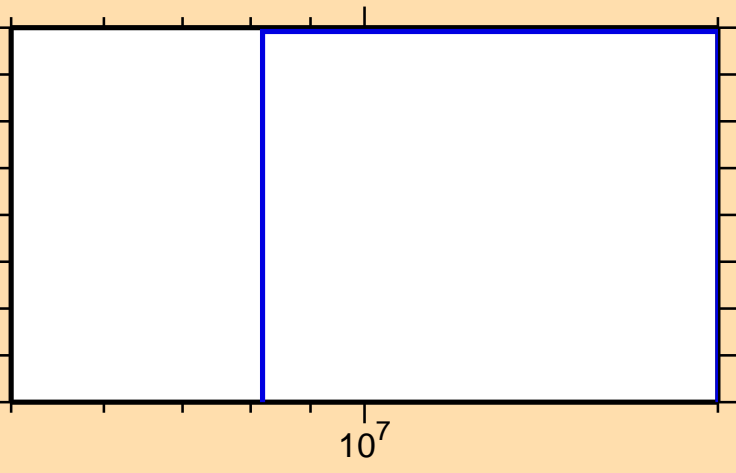
\sigma vs. E for ^{55}\text{V}(n,d)
