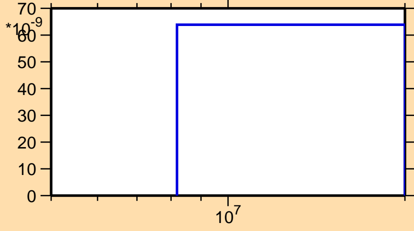
\sigma vs. E for ^{55}\text{V}(n,nt)
