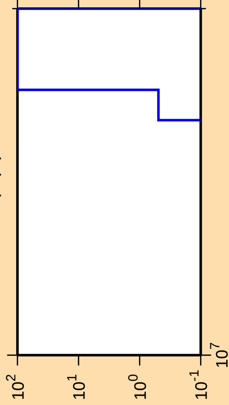
\Delta\sigma/\sigma vs. E for ^{172}\text{W}(n,\text{pt})
