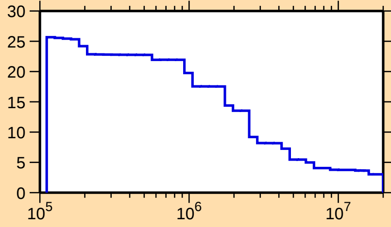
\Delta\sigma/\sigma vs. E for ^{172}\text{W}(\text{n,nonel.})
