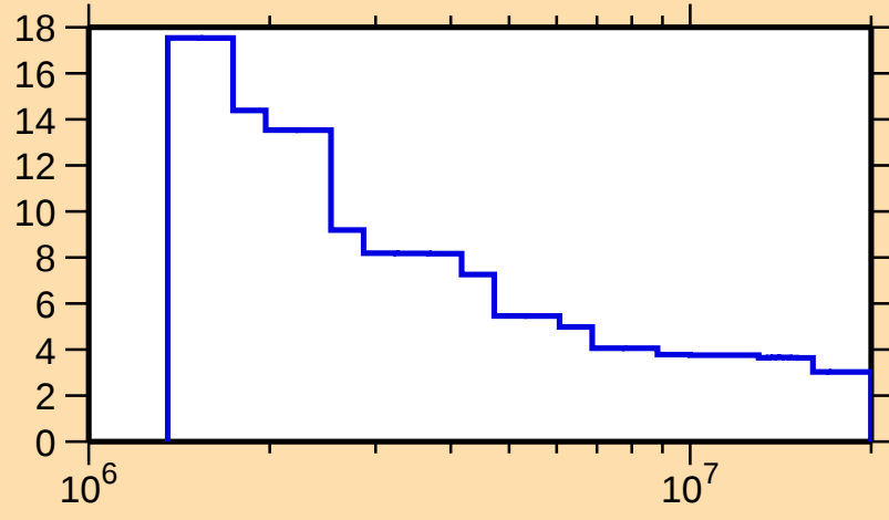
\Delta\sigma/\sigma vs. E for ^{172}\text{W}(\text{n},\text{nonel.})
