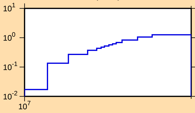
\sigma vs. E for ^{172}\text{W}(n,2n)
