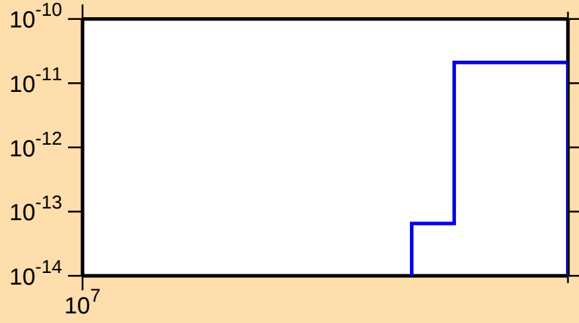
\sigma vs. E for ^{172}\text{W}(n,\text{pt})
