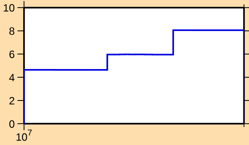
\Delta\sigma/\sigma vs. E for ^{172}\text{W}(n,\text{el.})
