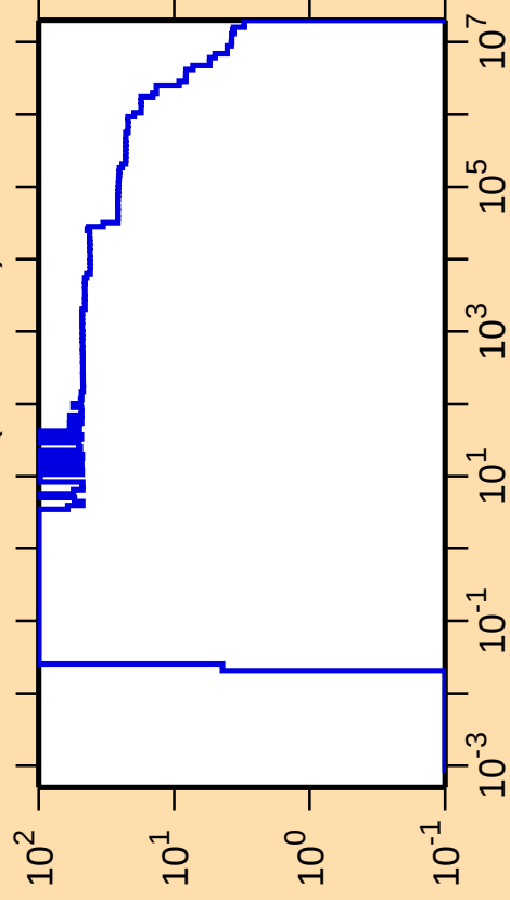
\Delta\sigma/\sigma vs. E for ^{172}\text{W}(\text{n,nonel.})
