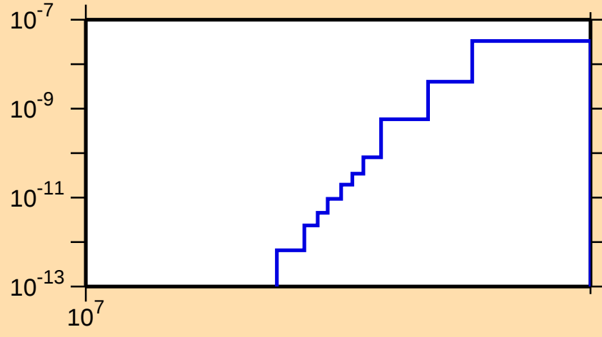
\sigma vs. E for ^{172}\text{W}(n,\text{pd})
