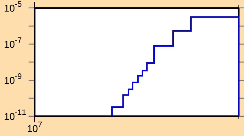
\sigma vs. E for ^{172}\text{W}(n,2n\alpha)
