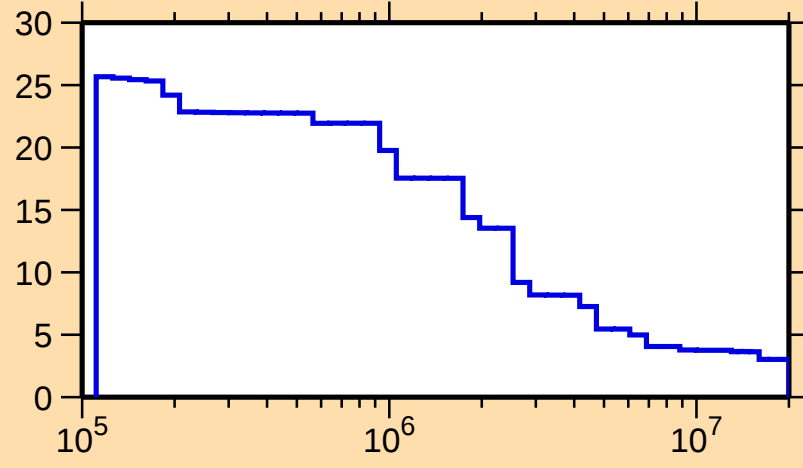
\Delta\sigma/\sigma vs. E for ^{172}\text{W}(n,\text{nonel.})
