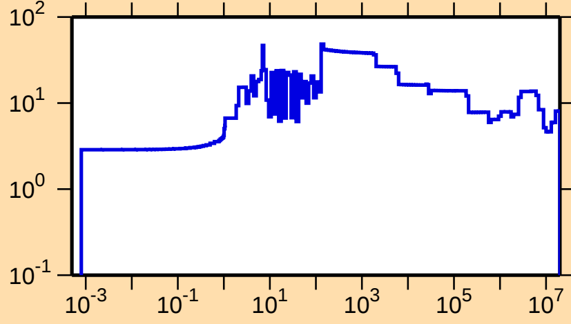
\Delta\sigma/\sigma vs. E for ^{172}\text{W}(n,\text{el.})
