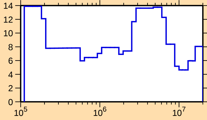
\Delta\sigma/\sigma vs. E for ^{172}\text{W}(\text{n,el.})
