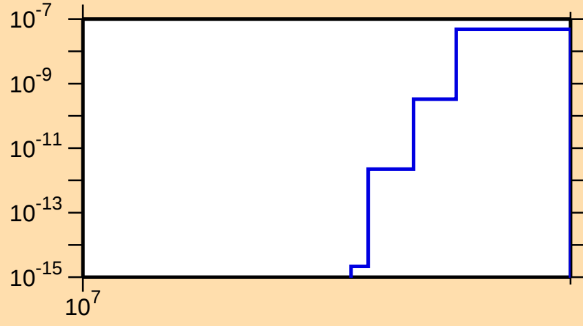
\sigma vs. E for ^{172}\text{W}(n,\text{nd})
