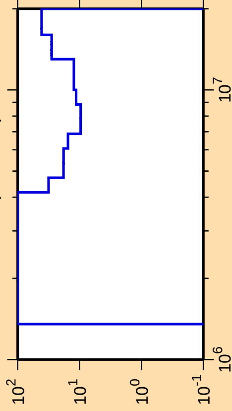
\Delta\sigma/\sigma vs. E for ^{172}\text{W}(\text{n},\text{ncont.})
