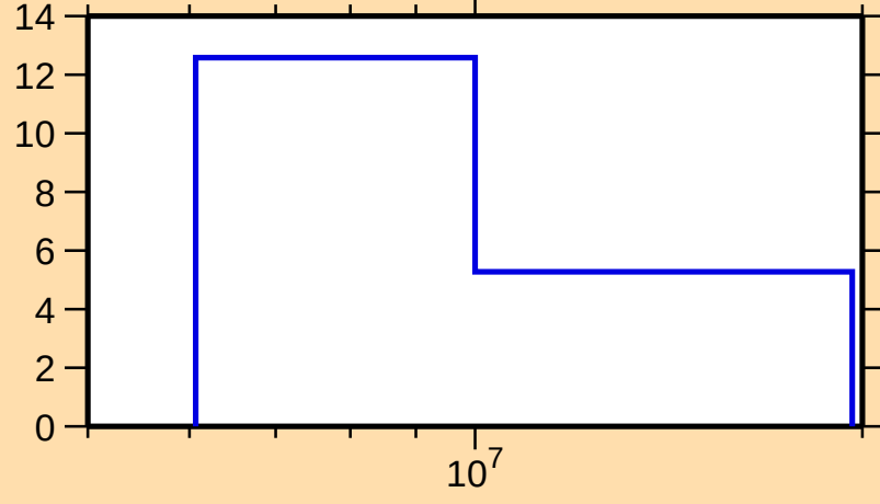
\Delta\sigma/\sigma vs. E for ^{176}\text{W}(n,\text{el.})
