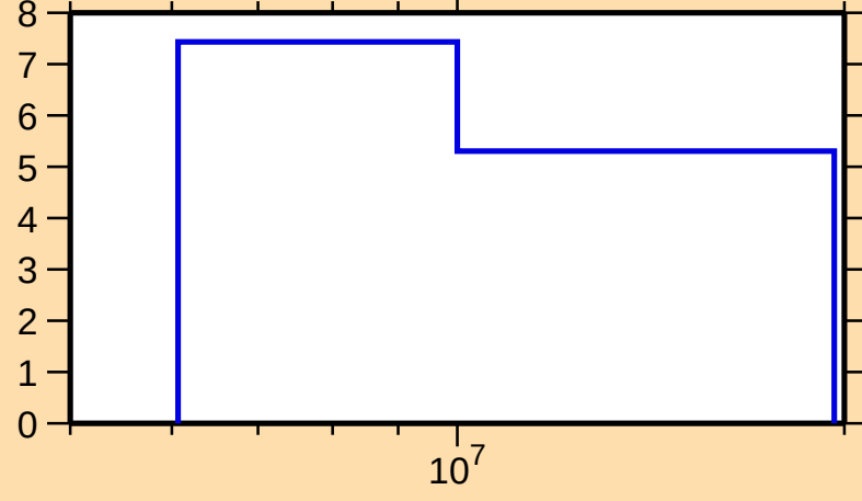
\Delta\sigma/\sigma vs. E for ^{176}\text{W}(n,\text{tot.})
