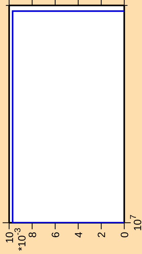
\Delta\sigma/\sigma vs. E for ^{176}\text{W}(n,\text{pt})
