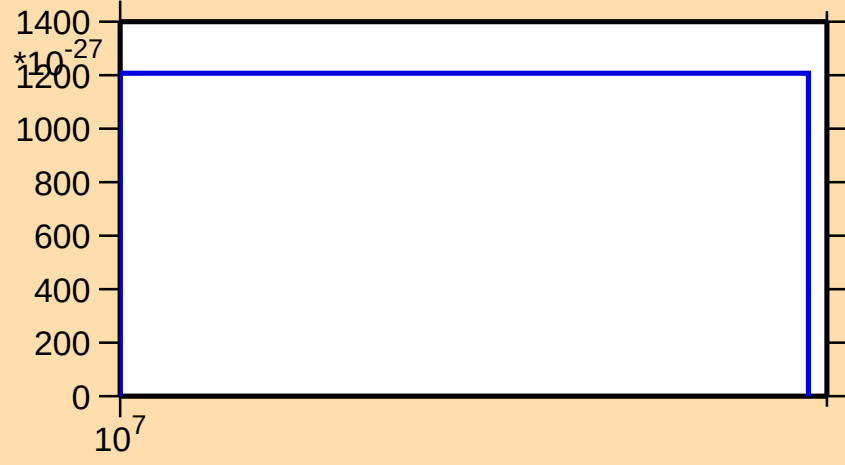
\sigma vs. E for ^{176}\text{W}(\text{mt 11})
