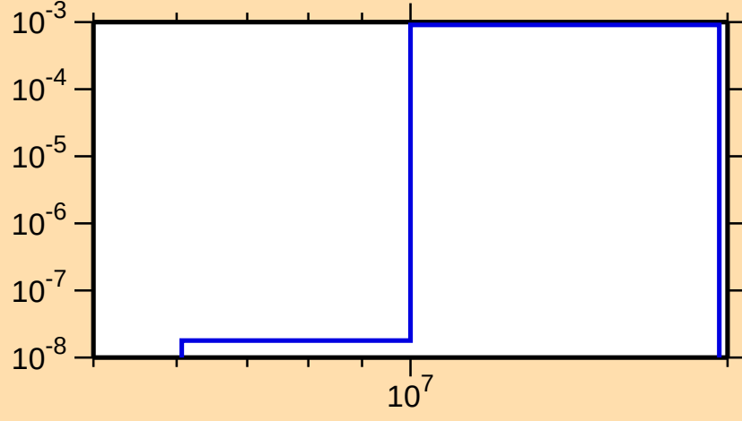
\sigma vs. E for ^{176}\text{W}(n,d)
