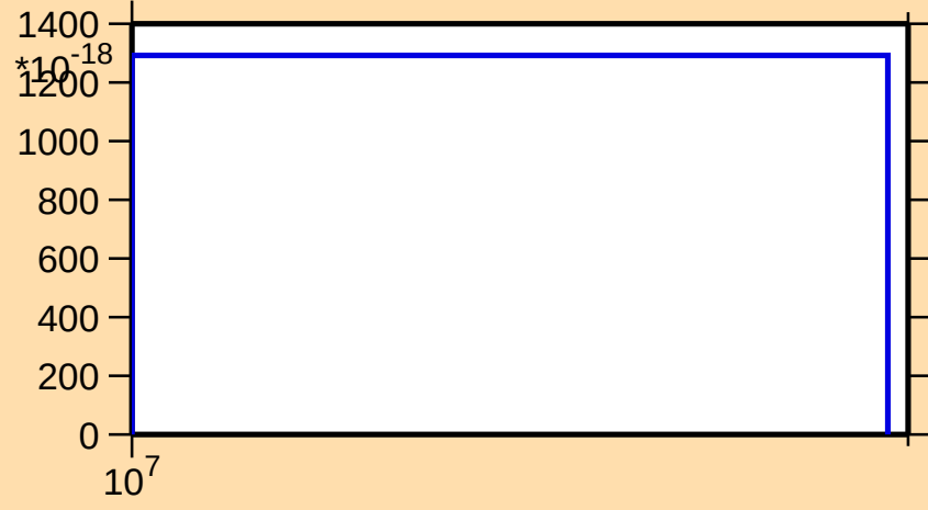
\sigma vs. E for ^{176}\text{W}(\text{mt } 34)
