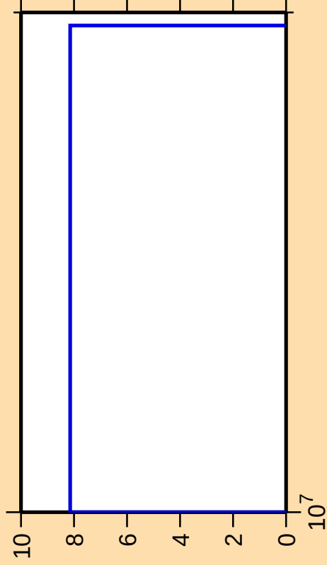
\Delta\sigma/\sigma vs. E for ^{176}\text{W}(n,\text{pd})
