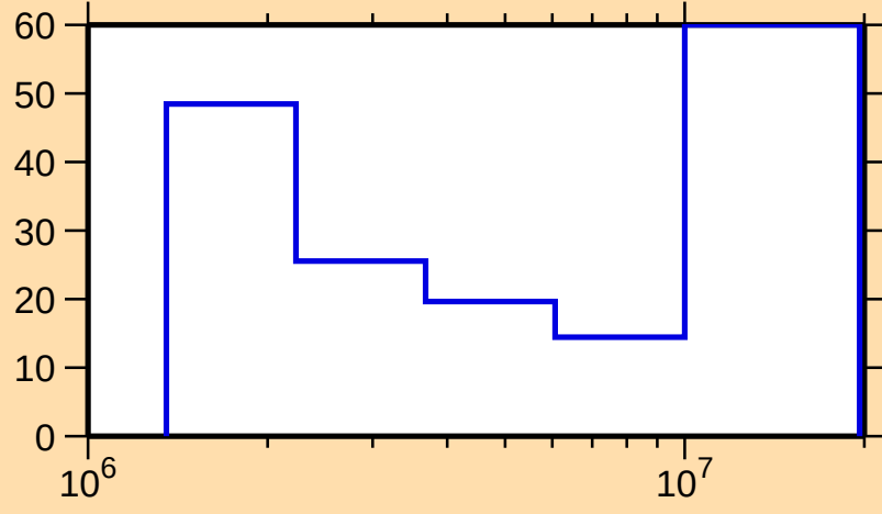
\Delta\sigma/\sigma vs. E for ^{176}\text{W}(n,n\text{cont.})
