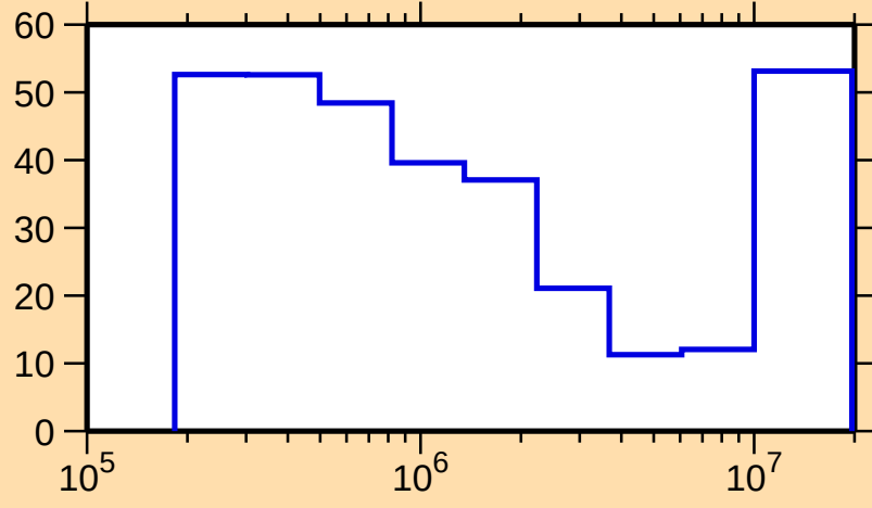
\Delta\sigma/\sigma vs. E for ^{176}\text{W}(n,\text{inel.})
