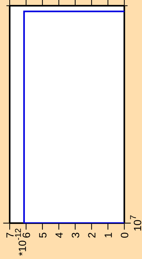
\Delta\sigma/\sigma vs. E for ^{176}\text{W}(\text{mt 11})
