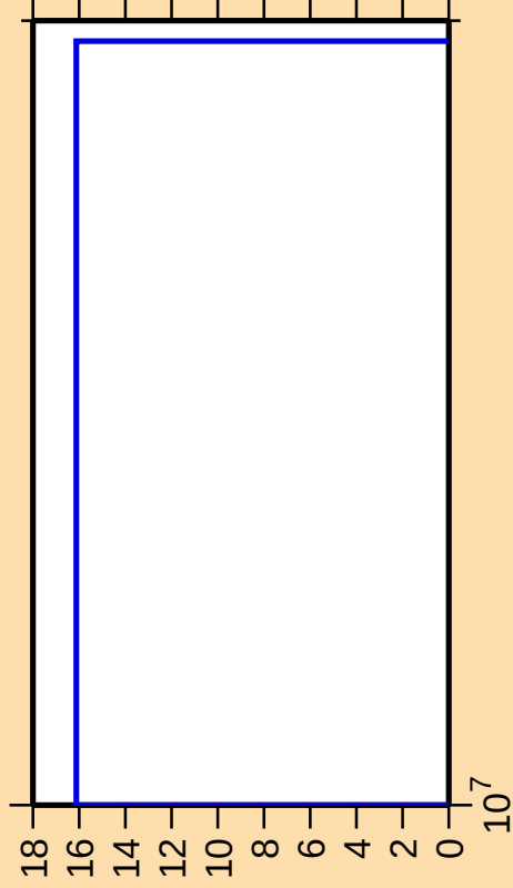
\Delta\sigma/\sigma vs. E for ^{176}\text{W}(\text{mt 45})
