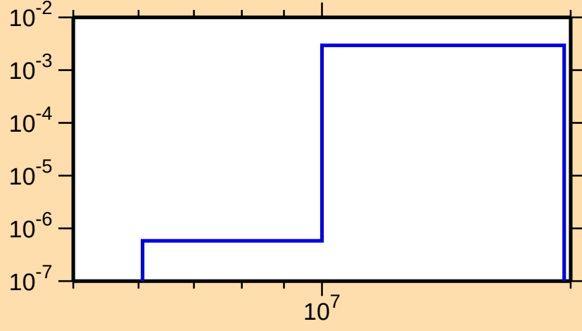
\sigma vs. E for ^{176}\text{W}(n,np)
