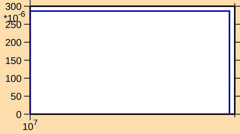
\sigma vs. E for ^{176}\text{W}(n,3n)
