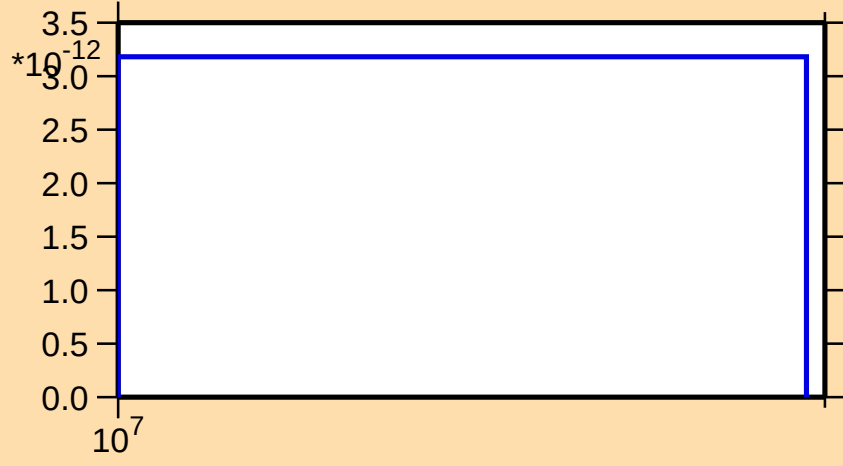
\sigma vs. E for ^{176}\text{W}(\text{mt 45})
