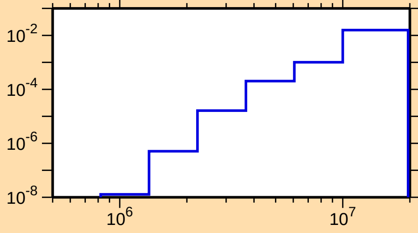
\sigma vs. E for ^{176}\text{W}(n,p)
