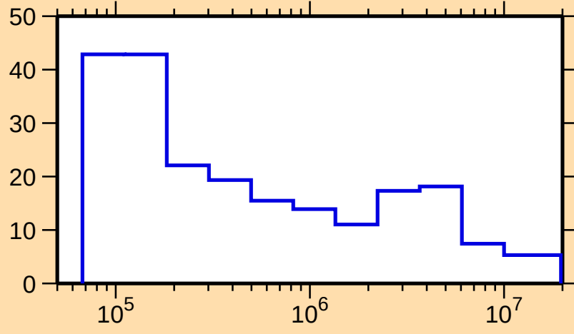
\Delta\sigma/\sigma vs. E for ^{176}\text{W}(n,\text{tot.})
