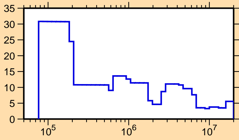
\Delta\sigma/\sigma vs. E for ^{177}\text{W}(n,\text{tot.})
