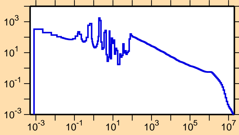
\sigma vs. E for ^{177}\text{W}(n,\gamma)
