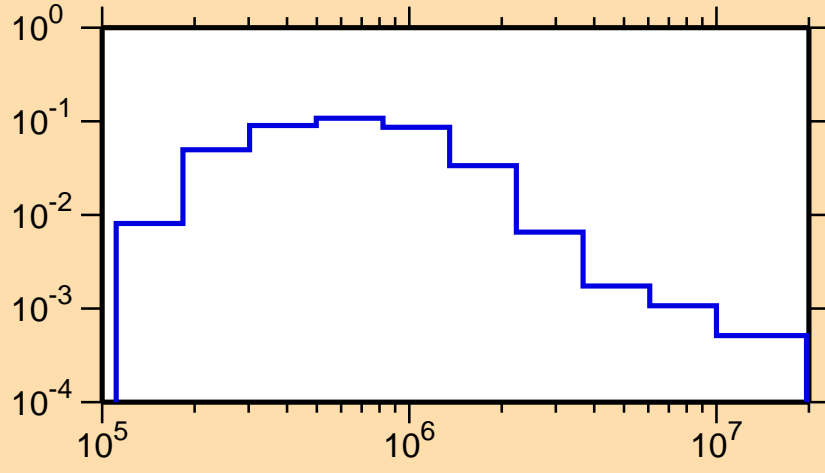
\sigma vs. E for ^{177}\text{W}(n,n_4)
