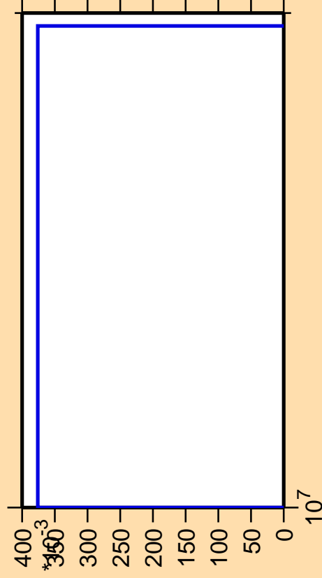
\Delta\sigma/\sigma vs. E for ^{177}\text{W}(n,\text{pd})
