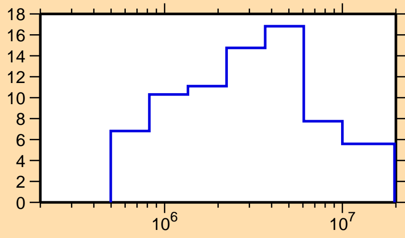
\Delta\sigma/\sigma vs. E for ^{177}\text{W}(n, el.)
