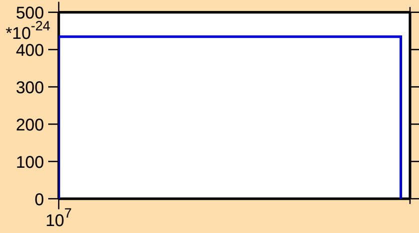
\sigma vs. E for ^{182}\text{W} (mt 11)
