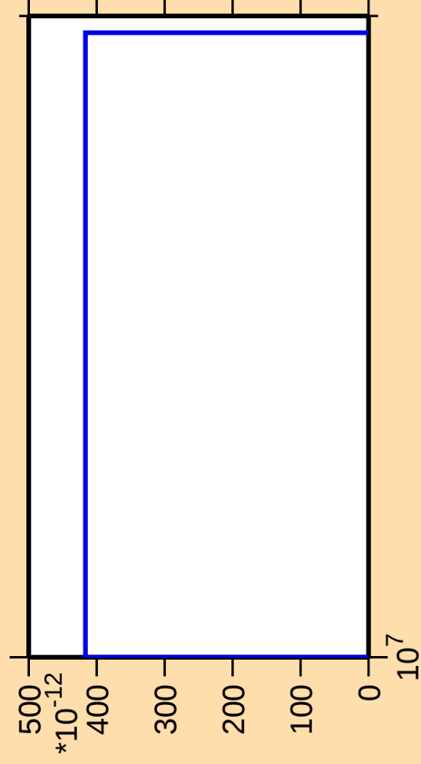
\Delta\sigma/\sigma vs. E for ^{182}\text{W} (mt 11)
