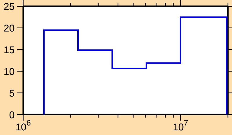
\Delta\sigma/\sigma vs. E for ^{182}\text{W}(\text{n},\text{el.})
