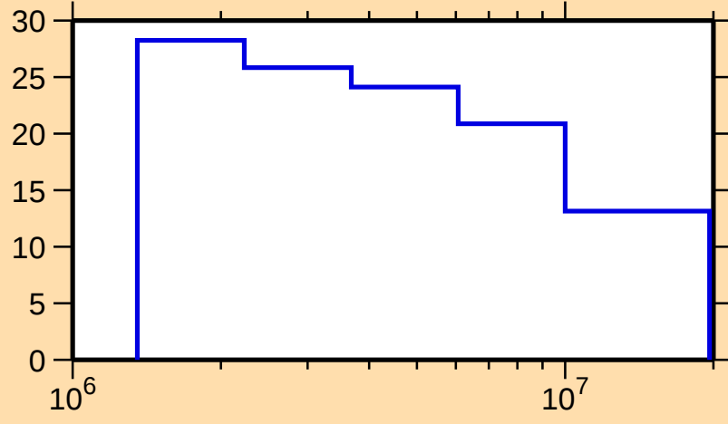
\Delta\sigma/\sigma vs. E for ^{182}\text{W}(n,\text{tot.})
