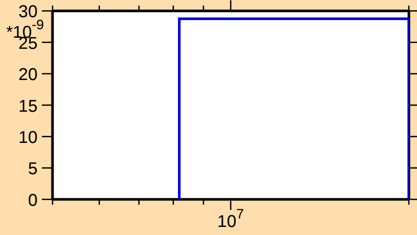
\sigma vs. E for ^{183}\text{W}(\text{n},\text{nd})
