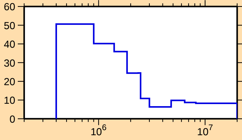
\Delta\sigma/\sigma vs. E for ^{183}\text{W}(\text{n,nonel.})
