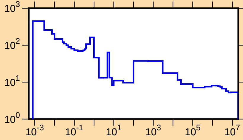
\sigma vs. E for ^{183}\text{W}(\text{n,tot.})
