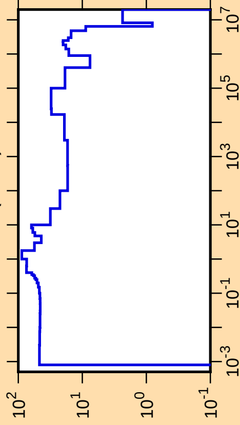
\Delta\sigma/\sigma vs. E for ^{183}\text{W}(\text{n,tot.})
