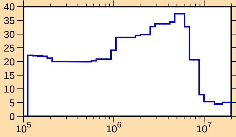
\Delta\sigma/\sigma vs. E for ^{184}\text{W}(\text{n,tot.})
