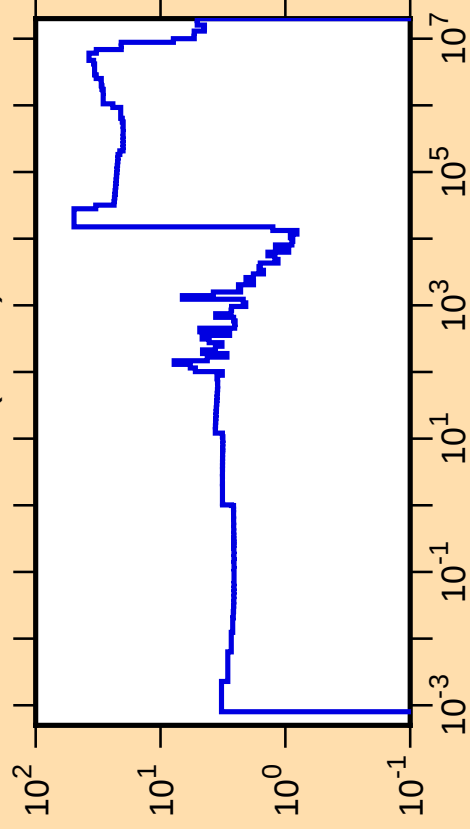
\Delta\sigma/\sigma vs. E for ^{184}\text{W}(n,\text{tot.})
