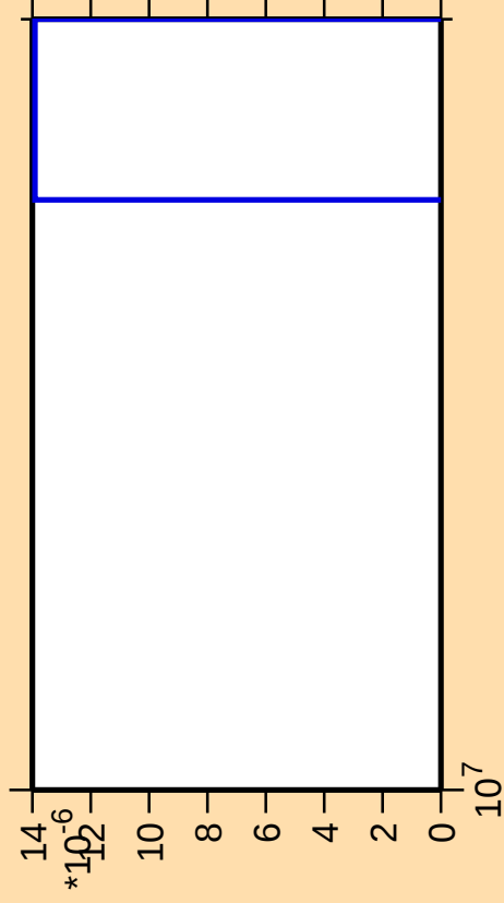
\Delta\sigma/\sigma vs. E for ^{184}\text{W}(\text{mt 11})
