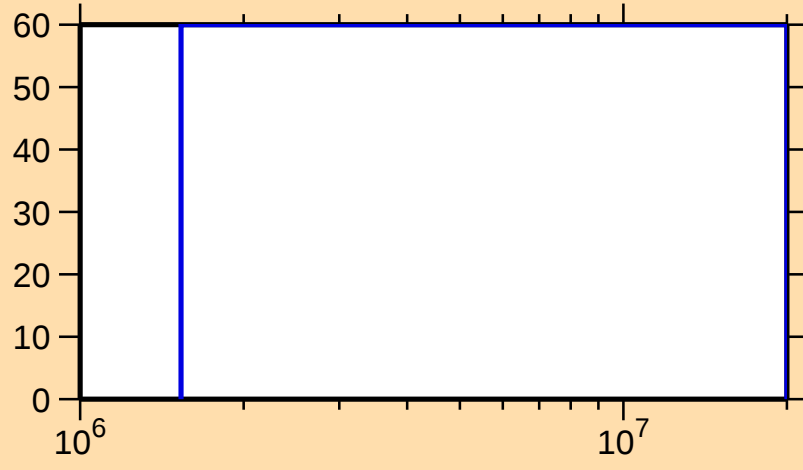
\Delta\sigma/\sigma vs. E for ^{184}\text{W}(\text{n,inel.})
