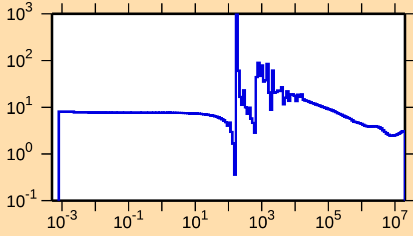
\sigma vs. E for ^{184}\text{W}(\text{n,el.})
