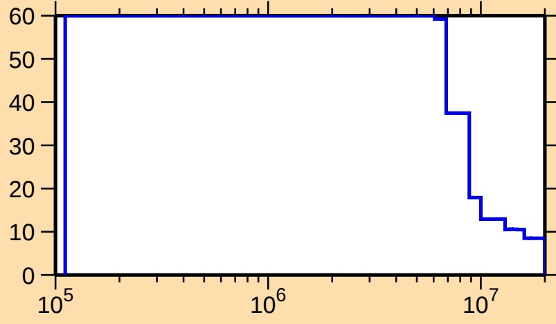
\Delta\sigma/\sigma vs. E for ^{184}\text{W}(\text{n,nonel.})
