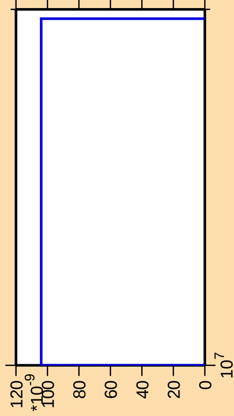
\Delta\sigma/\sigma vs. E for ^{184}\text{W}(\text{mt 11})
