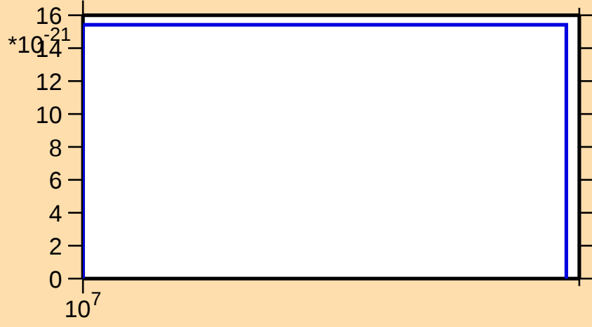
\sigma vs. E for ^{184}\text{W}(\text{mt 11})
