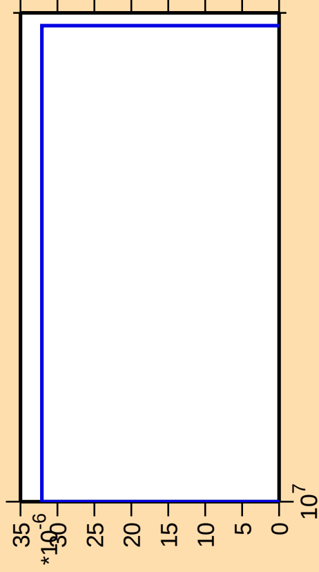
\Delta\sigma/\sigma vs. E for ^{184}\text{W}(n,3n\alpha)
