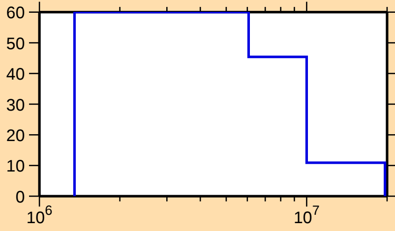
\Delta\sigma/\sigma vs. E for ^{184}\text{W}(\text{n},\text{nonel.})
