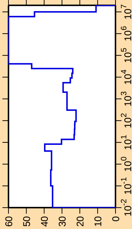
\Delta\sigma/\sigma vs. E for ^{184}\text{W}(\text{n,nonel.})
