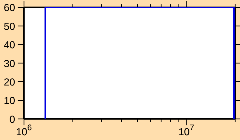
\Delta\sigma/\sigma vs. E for ^{184}\text{W}(\text{n},\text{inel.})
