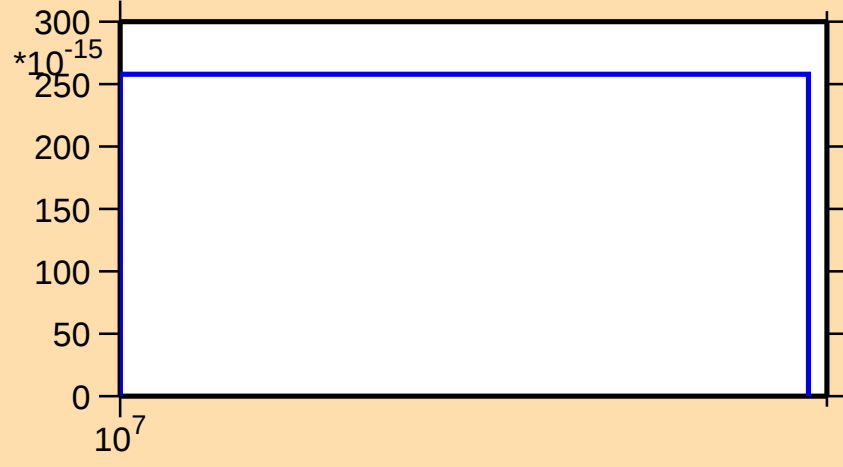
\sigma vs. E for ^{184}\text{W}(n,\text{He}3)
