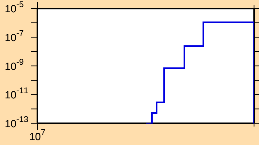
\sigma vs. E for ^{185}\text{W}(n,\text{nd})
