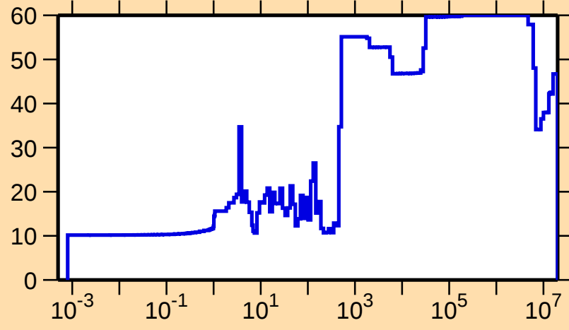
\Delta\sigma/\sigma vs. E for ^{185}\text{W}(n,\gamma)
