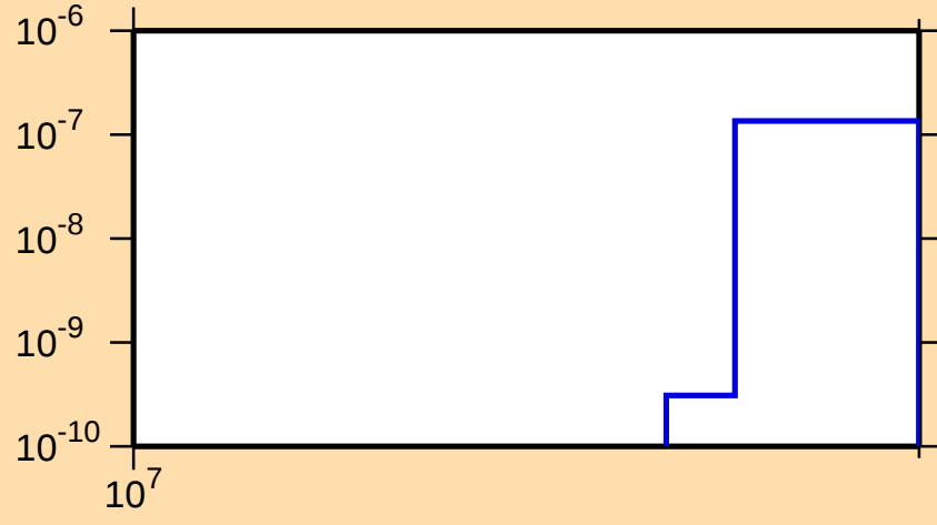
\sigma vs. E for ^{185}\text{W}(n,2np)
