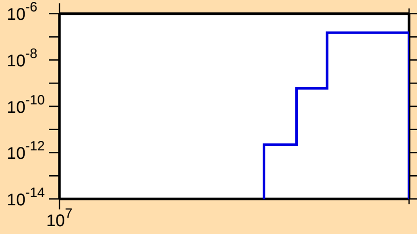
\sigma vs. E for ^{185}\text{W}(n,nt)
