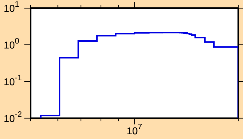
\sigma vs. E for ^{185}\text{W}(n,2n)
