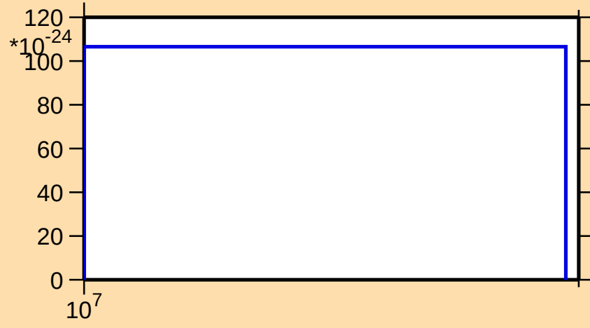
\sigma vs. E for ^{185}\text{W} (mt 11)
