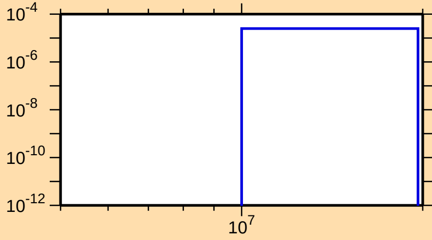
\sigma vs. E for ^{185}\text{W}(n,t)
