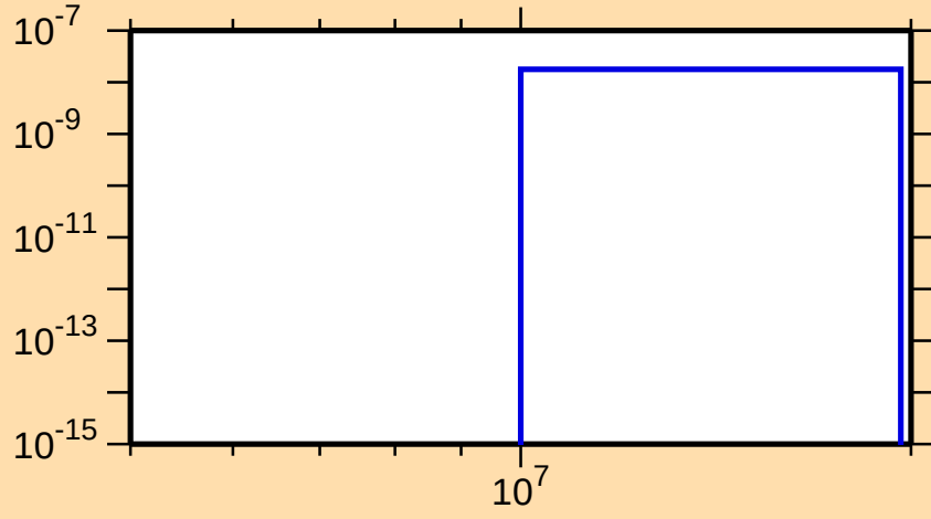
\sigma vs. E for ^{185}\text{W}(n,2n\alpha)
