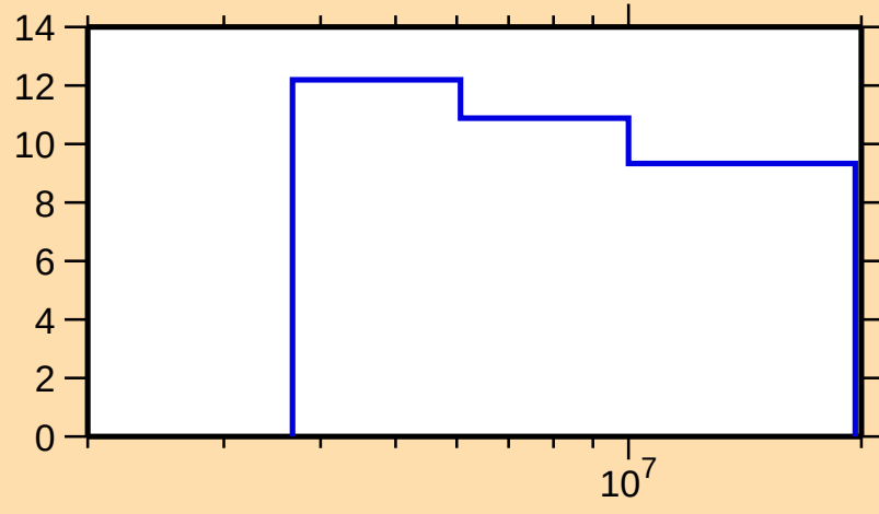
\Delta\sigma/\sigma vs. E for ^{185}\text{W}(n,\text{nonel.})
