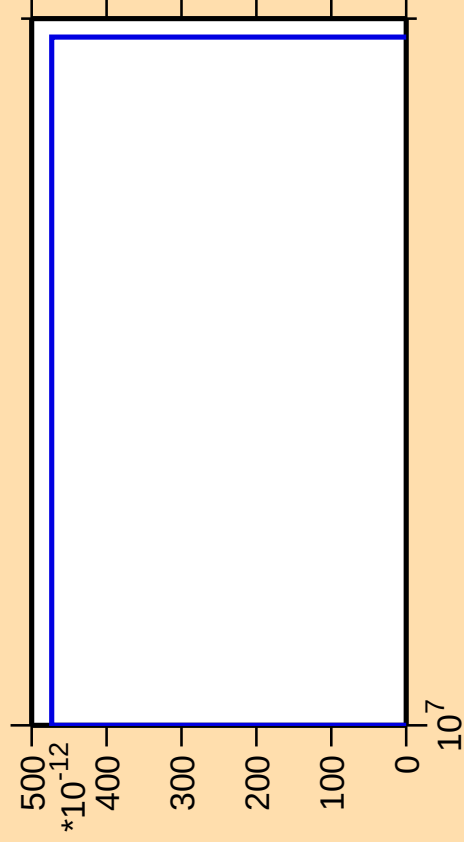
\Delta\sigma/\sigma vs. E for ^{185}\text{W} (mt 11)
