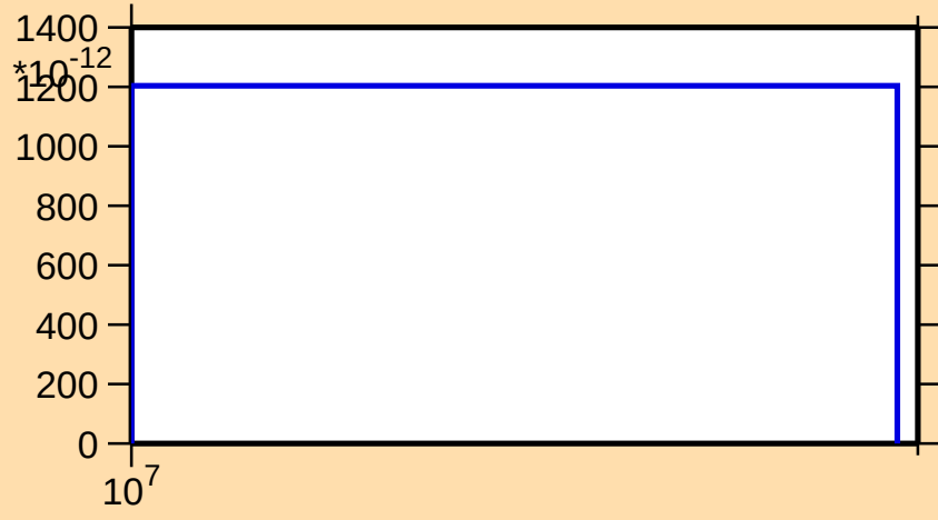
\sigma vs. E for ^{185}\text{W}(n,\text{nt})
