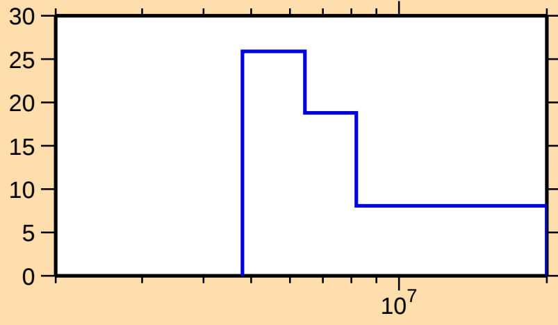
\Delta\sigma/\sigma vs. E for ^{185}\text{W}(n,\text{el.})
