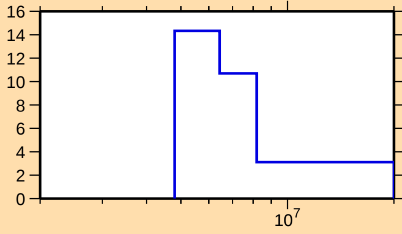
\Delta\sigma/\sigma vs. E for ^{185}\text{W}(n,\text{tot.})
