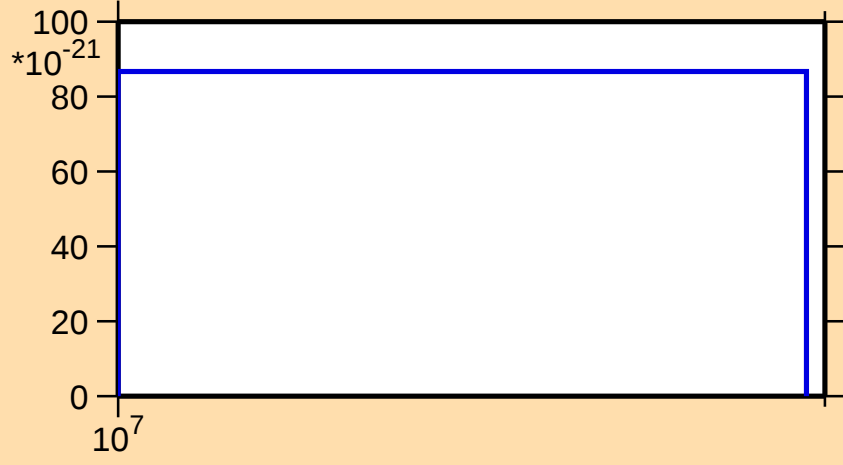
\sigma vs. E for ^{188}\text{W}(\text{mt 11})
