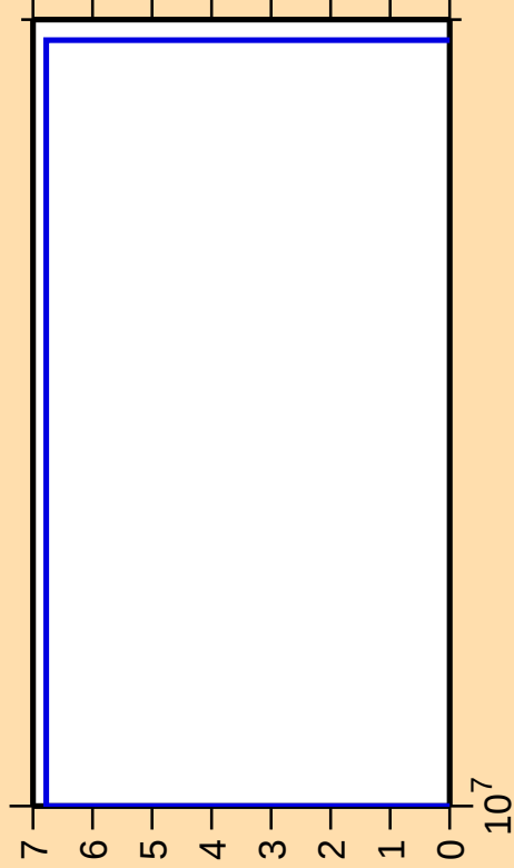
\Delta\sigma/\sigma vs. E for ^{188}\text{W}(n,2np)
