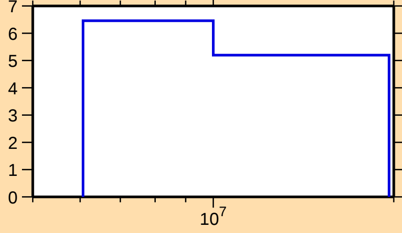
\Delta\sigma/\sigma vs. E for ^{188}\text{W}(n,\text{tot.})
