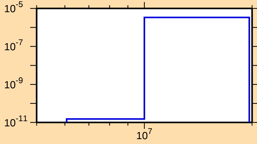
\sigma vs. E for ^{188}\text{W}(n,n\alpha)
