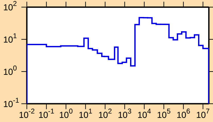
\Delta\sigma/\sigma vs. E for ^{188}\text{W}(\text{n,tot.})
