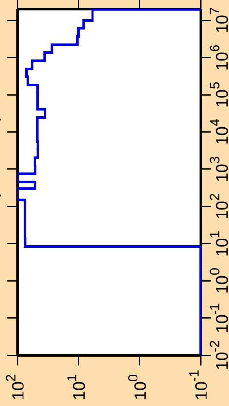
\Delta\sigma/\sigma vs. E for ^{188}\text{W}(\text{n,nonel.})
