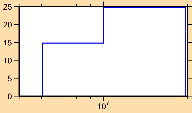
\Delta\sigma/\sigma vs. E for ^{192}\text{W}(n,2n)
