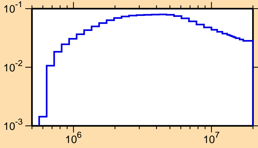
\sigma vs. E for ^{113}\text{Xe}(n,n_4)
