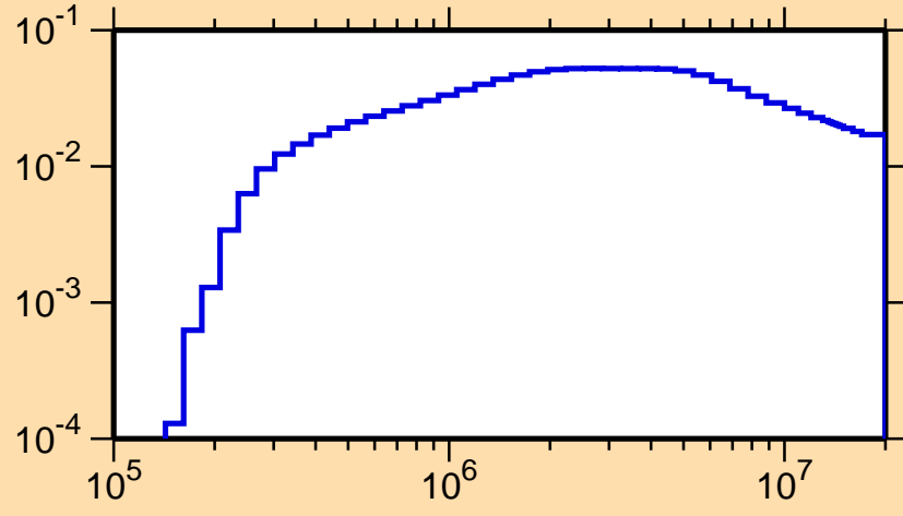
\sigma vs. E for ^{113}\text{Xe}(n,n_2)
