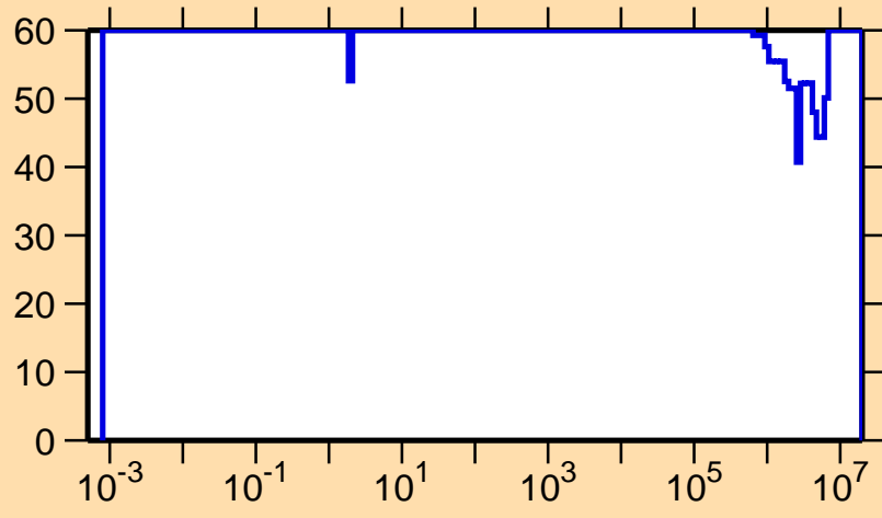
\Delta\sigma/\sigma vs. E for ^{113}\text{Xe}(n,\gamma)
